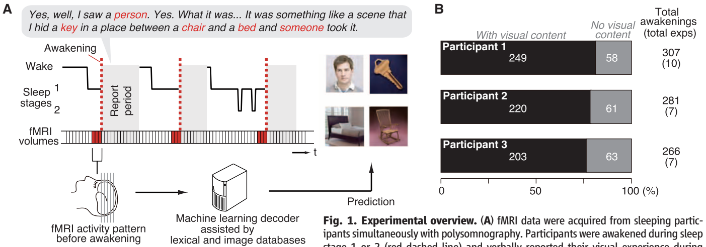
Fig. 1. Experimental overview. (A) fMRI data were acquired from sleeping participants simultaneously with polysomnography. Participants were awakened during sleep stage 1 or 2 (red dashed line) and verbally reported their visual experience during sleep. fMRI data immediately before awakening [an average of three volumes (= 9 s)] were used as the input for main decoding analyses (sliding time windows were used for time course analyses). Words describing visual objects or scenes (red letters) were extracted. The visual contents were predicted using machine-learning decoders trained on fMRI responses to natural images. (B) The numbers of awakenings with and without visual contents are shown for each participant (with numbers of experiments in parentheses).
