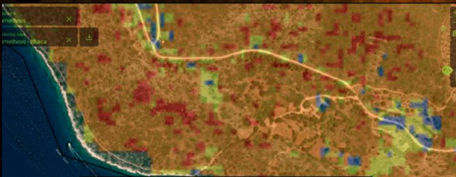
Island of Ithaca High-Resolution details of extreme events forecast
