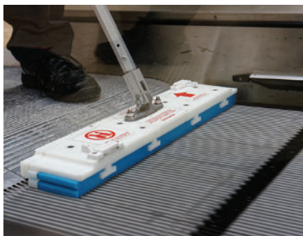
REN system is used for daily cleaning (escalator maintenance)
