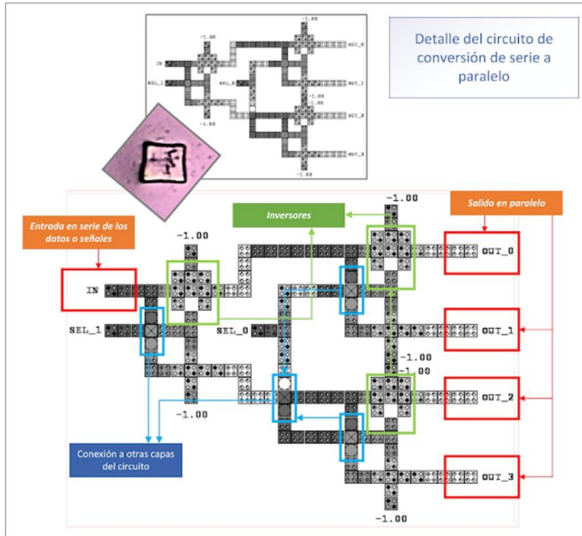
Fig. 7. Details of the circuit for converting TS-OOK signals in series to a parallel output, confirming one of the typical tasks of a router. (Sardinha, LH; Costa, AM; Neto, OPV; Vieira, LF; Vieira, MA 2013)
