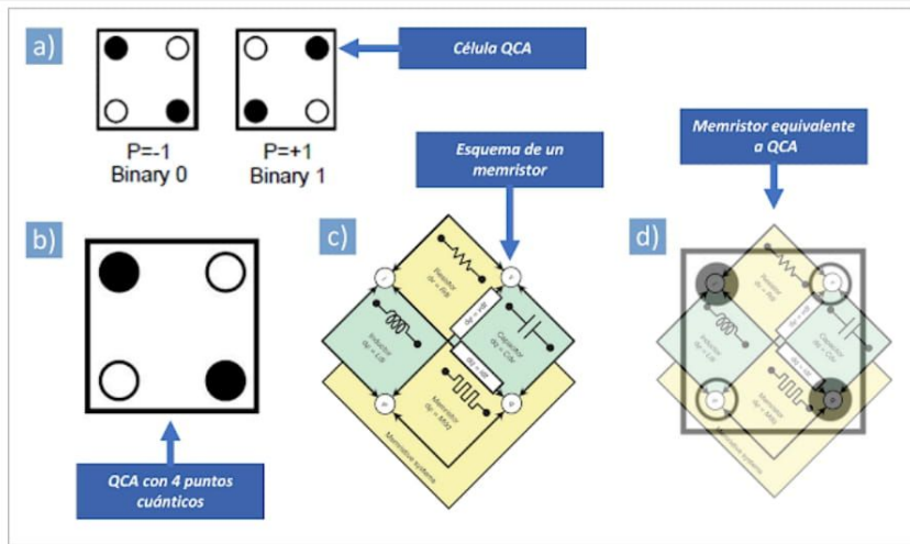
Fig. 4. Scheme of a QCA cell made up of four quantum dots (which can be graphene, among other materials). Note the great resemblance to memristors, in fact QCA's and memristors are transistors. (Sardinha, LH; Costa, AM; Neto, OPV; Vieira, LF; Vieira, MA 2013 | Strukov, DB; Snider, GS; Stewart, DR; Williams, RS 2009)
