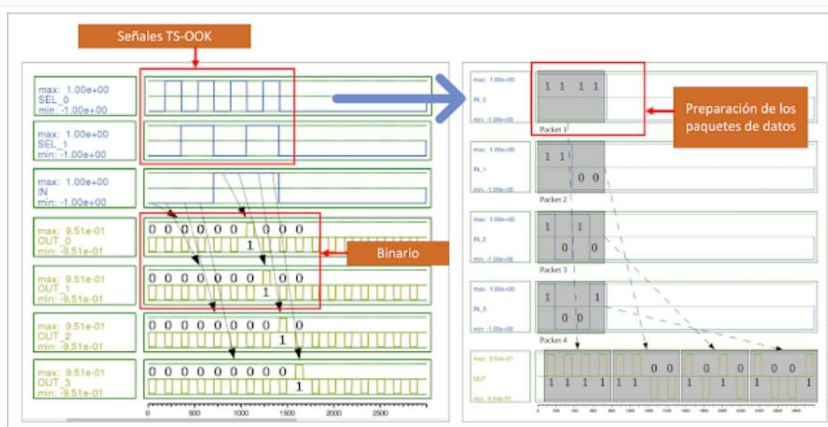
Fig. 8. The tests of the demux circuit, already observed in figure 7, provide the proof of how the TS-OOK signals are interpreted and converted to the binary code, to finally generate the data packets of the corresponding nanocommunications protocol. (Sardinha, LH; Costa, AM; Neto, OPV; Vieira, LF; Vieira, MA 2013)
