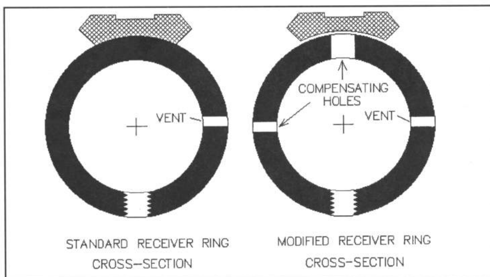
Figure 4-19 - Lateral cross-section view of the forward receiver ring and scope mount base showing modifications made to improve symmetry.
