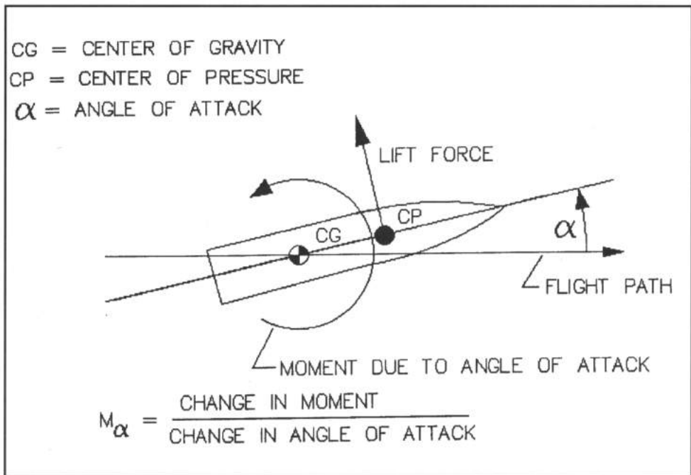
Figure 10-7 - Sketch showing how the lift force acting forward of the center of gravity results in a nose up unstable moment about the CG.
