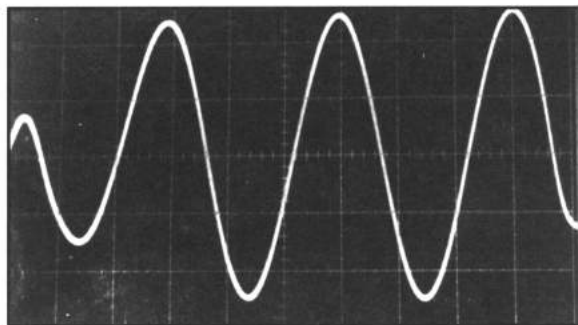
Figure 8-8 - Photograph of an oscilloscope trace showing the sine wave signal generated in the magnetometer coil by the rotating magnet in the nose of the bullet. Horizontal time scale is 0.1 msec per cm. Voltage scale is 0.1 volt per cm.
