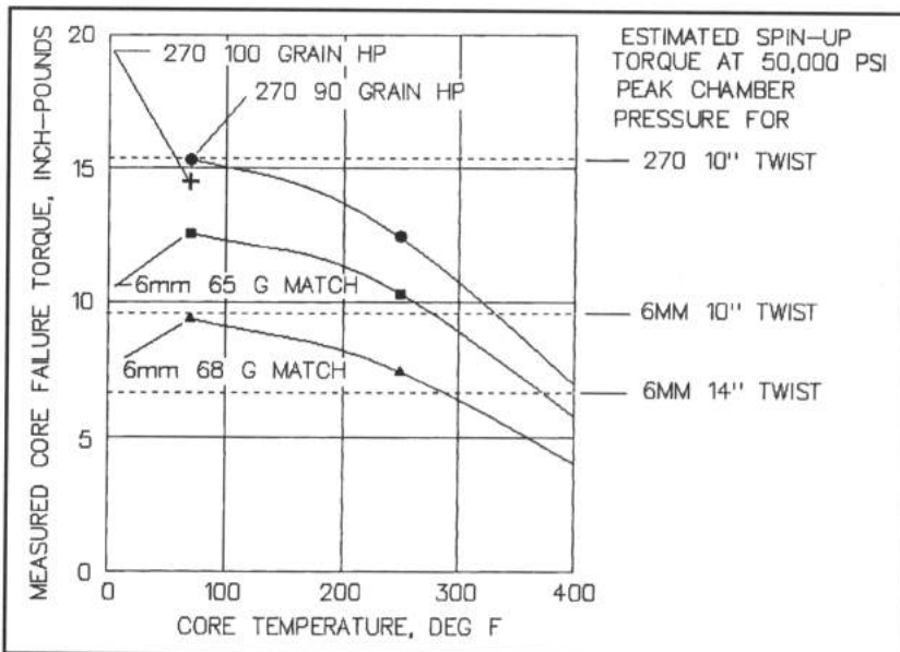
Figure 8-4 - Core failure torque for the four test bullets at normal and elevated temperatures.
