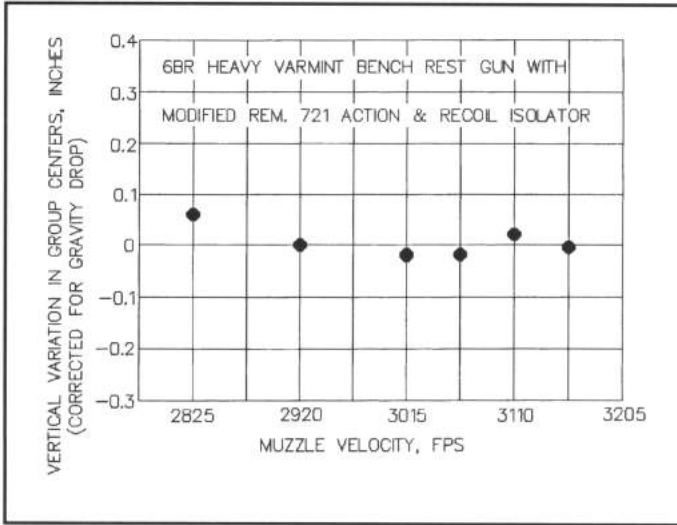
Figure 4-42 - Plot of the vertical positions of 5 shot group centers for various loads and muzzle velocities in the modified 721 action with recoil isolator and heavy varmint 6mm BR barrel. Gravity drop variation is removed.
