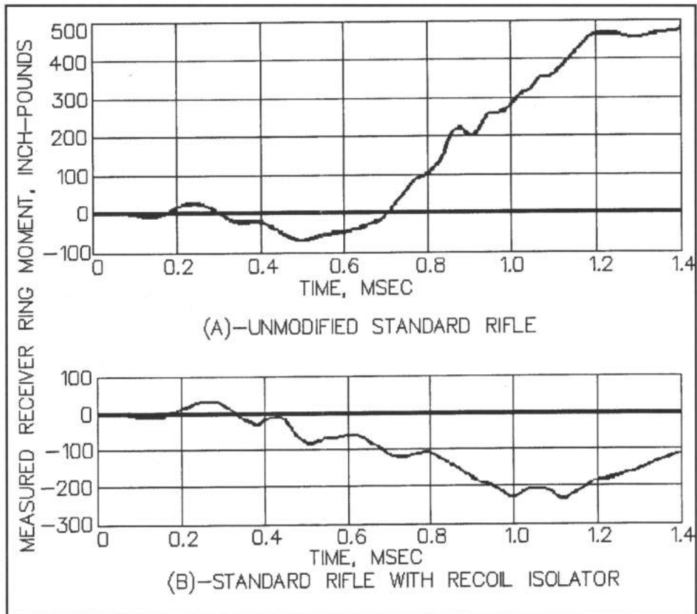
Figure 4-9 - Experimental receiver ring moment for the standard rifle (A) and the standard rifle with the Recoil Isolator (B).
