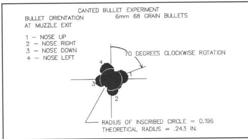
Figure 7-12 - Computer scan of the target where four groups of 4 bullets each that were canted 0.215 degrees in the case neck. The bullets were indexed in 90 degree intervals in roll. The radius of dispersion of 0.196 inches is superimposed. The trajectory simulation predicted 0.243 inches for radius of dispersion.
