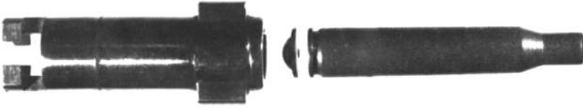
Figure 4-10 - Photograph of the rifle bolt with swiveling bolt face that proved to be unnecessary.
