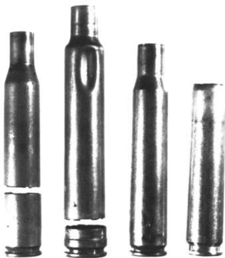
Figure 2-26 - Photograph of four cartridge cases showing different modes of failure. Head separation is shown on the first two cases from the left. Axial split near the head on the third case from the left. The case on the right resulted from firing a 7mm-08 in a 280 Remington chamber.
