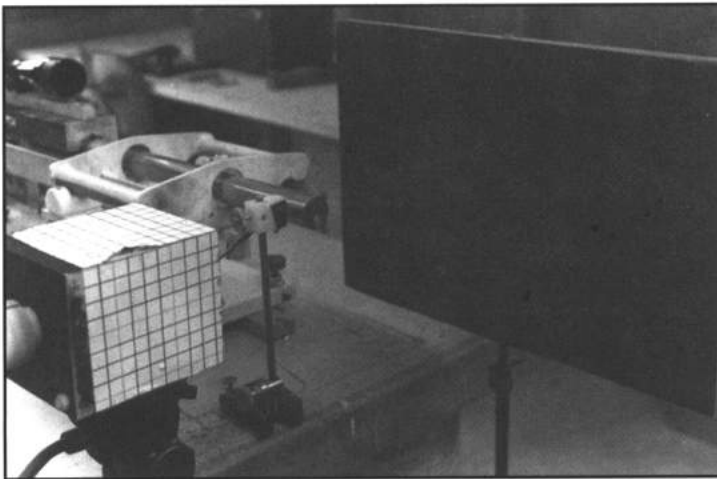
Figure G-3 - Front view of the shadowgraph setup, showing the arc light source on the left and the film mounting board on the right. The microphone is placed near the muzzle for late time shots.
