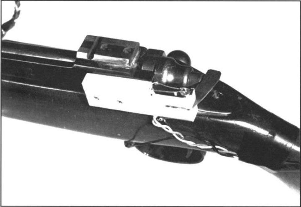
Figure 2-14 - Photograph of the scope trigger switch that starts the instrumentation.
