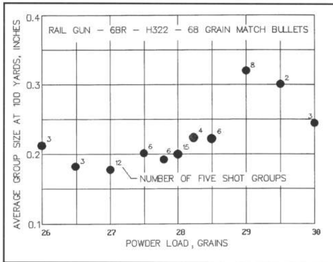
Figure 4-40 - Graph showing 5 shot group size from the rail gun in the Tunnel Range with different powder loads.
