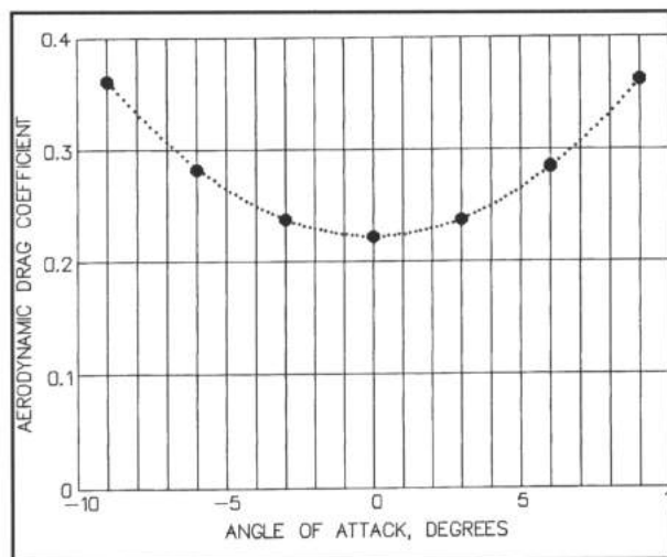
Figure 10-20 - Graph showing how the aerodynamic drag on an ogive cylinder bullet varies with angle of attack. The aerodynamic drag is very insensitive to small changes in angle of attack. From the tests in Chapter 7 we know that the angle of attack at muzzle exit is much less than one degree. A one degree angle increases the drag coefficient and decreases the ballistic coefficient by less than one percent.
