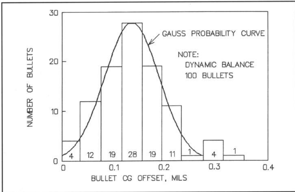
Figure C-4 - CG offset data for 100 bullets obtained from the dynamic balance device compared to a standard Gaussian distribution.
