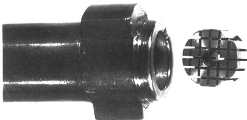
Figure 4-13 - Photograph of bolt head insert that allows lateral translation of cartridge case head.
