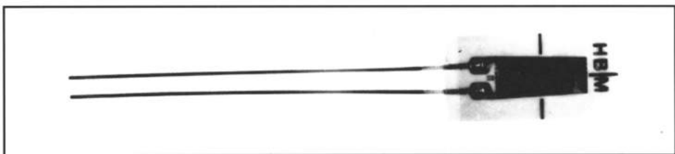
Figure 2-4 - Photograph of a strain gage similar to those used in chamber pressure and receiver ring moment experimental measurements. Actual size is 0.25 by 0.50 inches.
