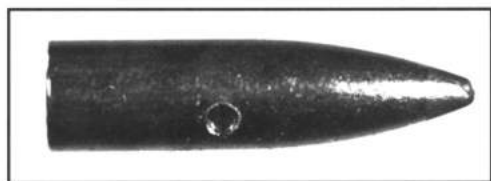
Figure 9-2 - Photograph of a 270 bullet modified by drilling a hole to deliberately produce an exaggerated CG offset of 0.00118 inches.
