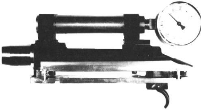
Figure 5-3 - Photograph of the hydraulic cylinder used to impose a compression force of up to 200 pounds between the front and rear mounts. Muzzle deflection was measured by dial gages.
