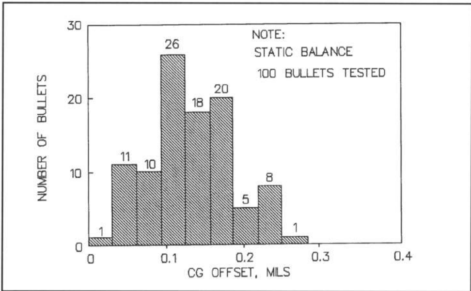
Figure 9-5 - Bar chart showing the results obtained in checking the static balance of a box of 100 caliber 270 bullets.
