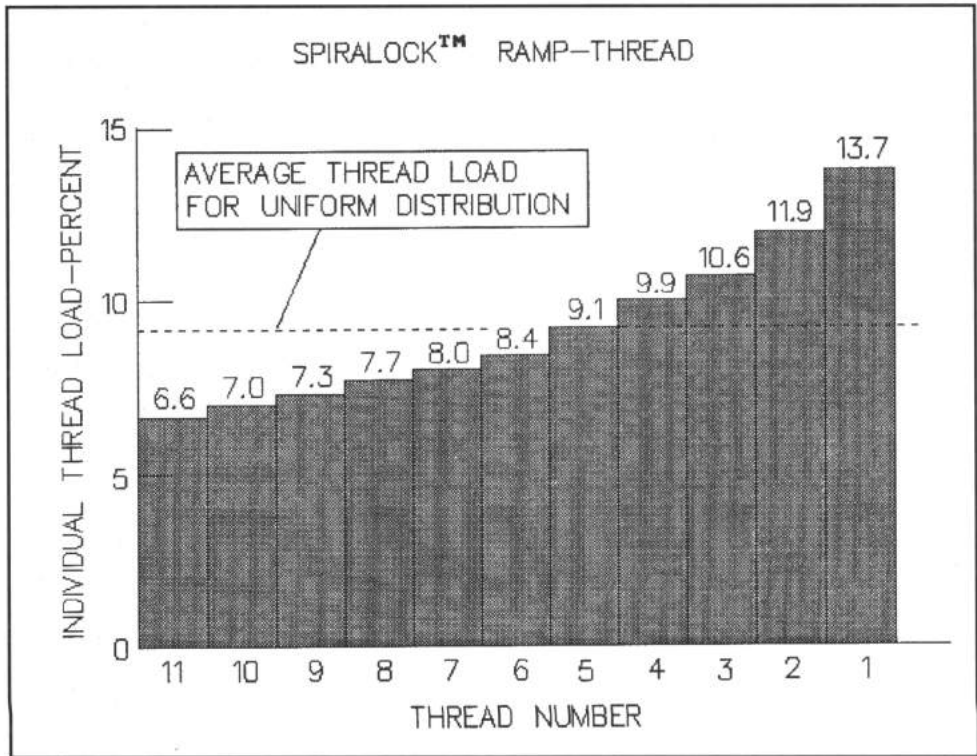
Figure 6-9 - Calculated individual thread load for the Spirallock™ ramp-thread in terms of percentage of total preload. The load distribution is much more evenly distributed than was the case with the standard thread (Figure 6-6).
