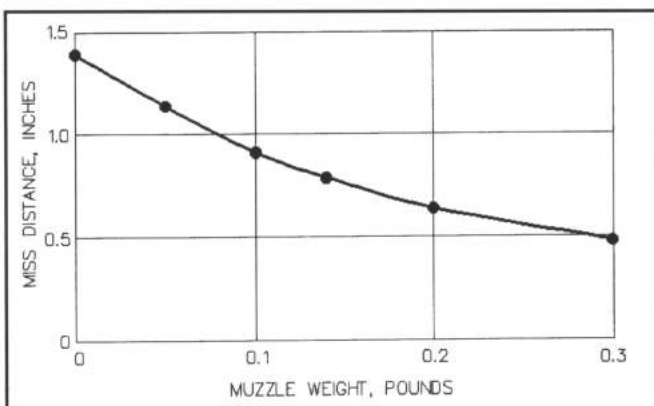
Figure 4-37 - Calculated effect of a muzzle weight on the miss distance due to reduction in barrel vibration. A small muzzle weight theoretically reduces barrel vibration significantly.
