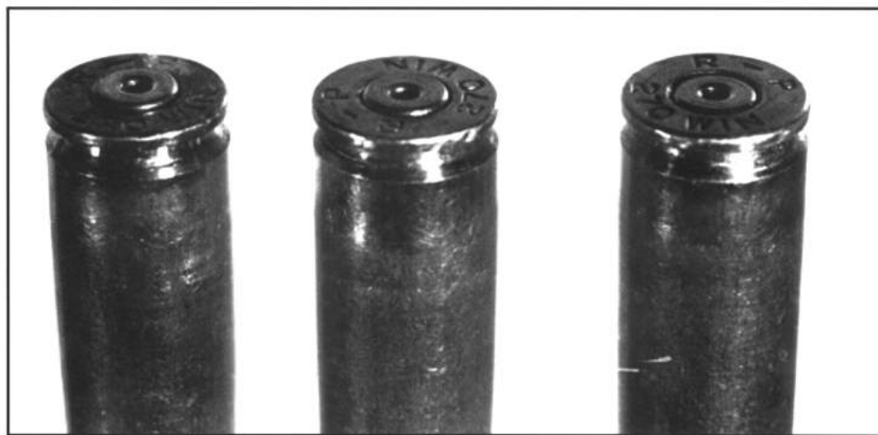
Figure 4-15 - Photograph of fired 270 Winchester cases showing primer protrusion resulting from excess headspace of 15, 8, and 0 mils from left to right. Experiment is performed with special work hardened and degreased cases.
