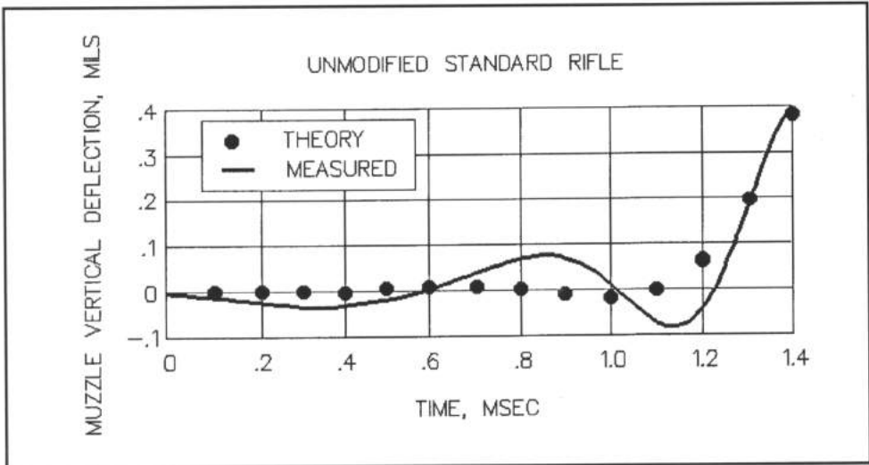
Figure 4-32 - Comparison of the measured experimental muzzle vertical deflection for the unmodified standard rifle to the calculated muzzle vertical deflection from the barrel vibration computer code.
