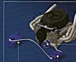
3 Energy storage system Weight: approx 14.5kg. The Li-on batteries are housed in a Zylon casing for safety
