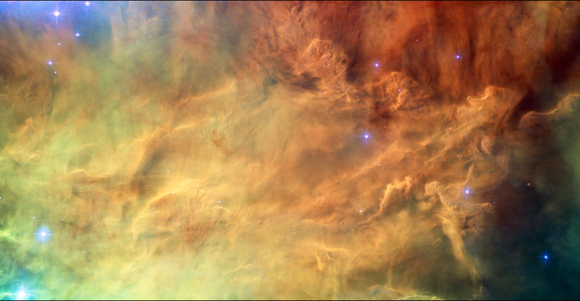
Lagoon Nebula star-forming molecular cloud
