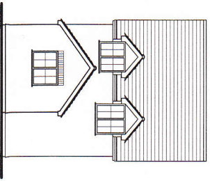
Proposed Rear Elevation scale 1:100
