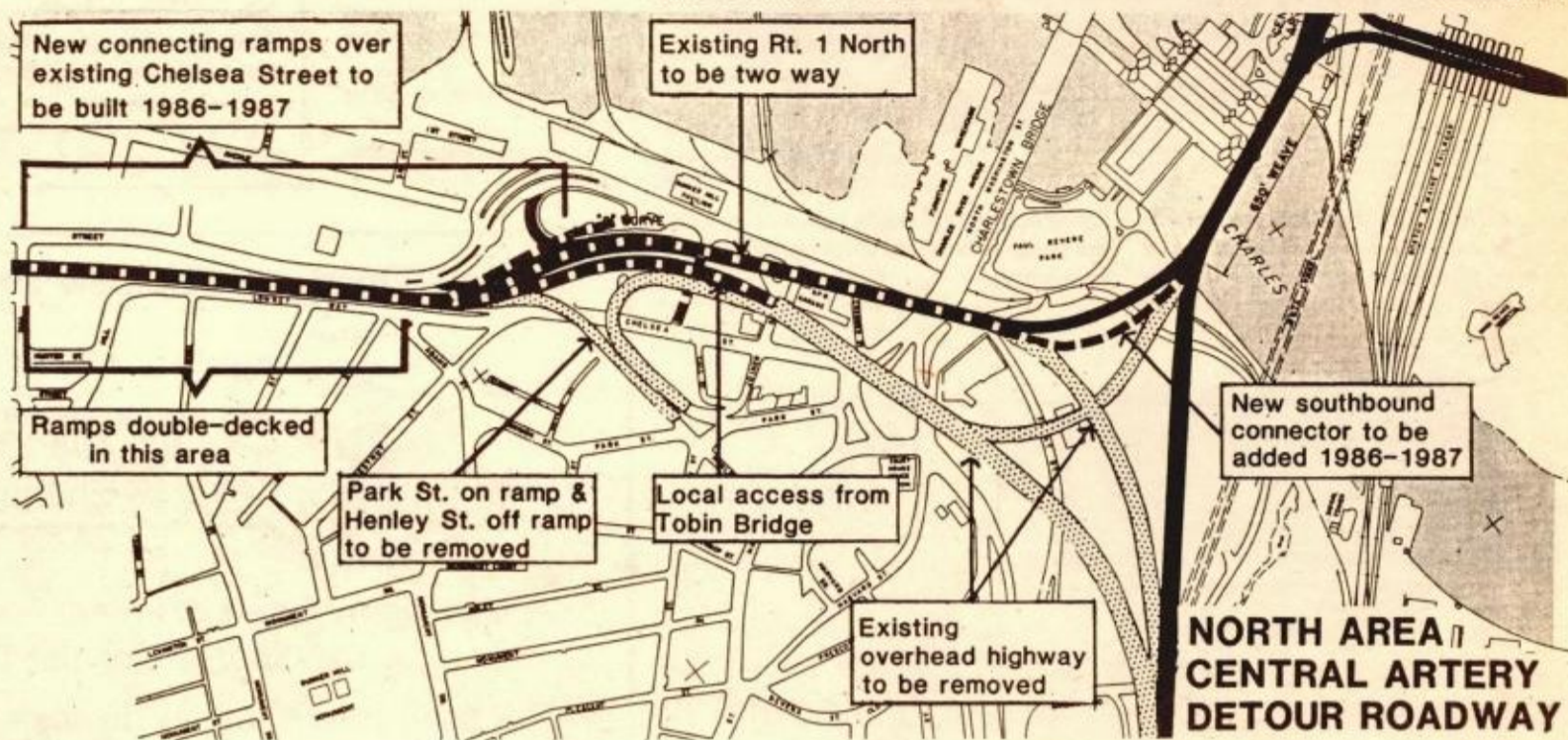
THE ABOVE PLAN show the proposed detour roadways to be built as part of the North Area / Central Artery project. Beginning in 1986, new ramps connecting the existing Route 1 north to the Tobin Bridge will be built. Route 1 north will become two-way and when the new connecting ramps are completed, traffic will be removed from the existing Route 1 south, the ramps will be removed and the tunnels under City Square will be constructed.
