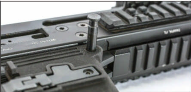
The two takedown pins work just like those on an AR-15.
