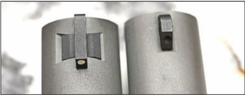
On the left, the new Delta with its Novak front sight, and on the right the old model, with a staked-in front sight.
