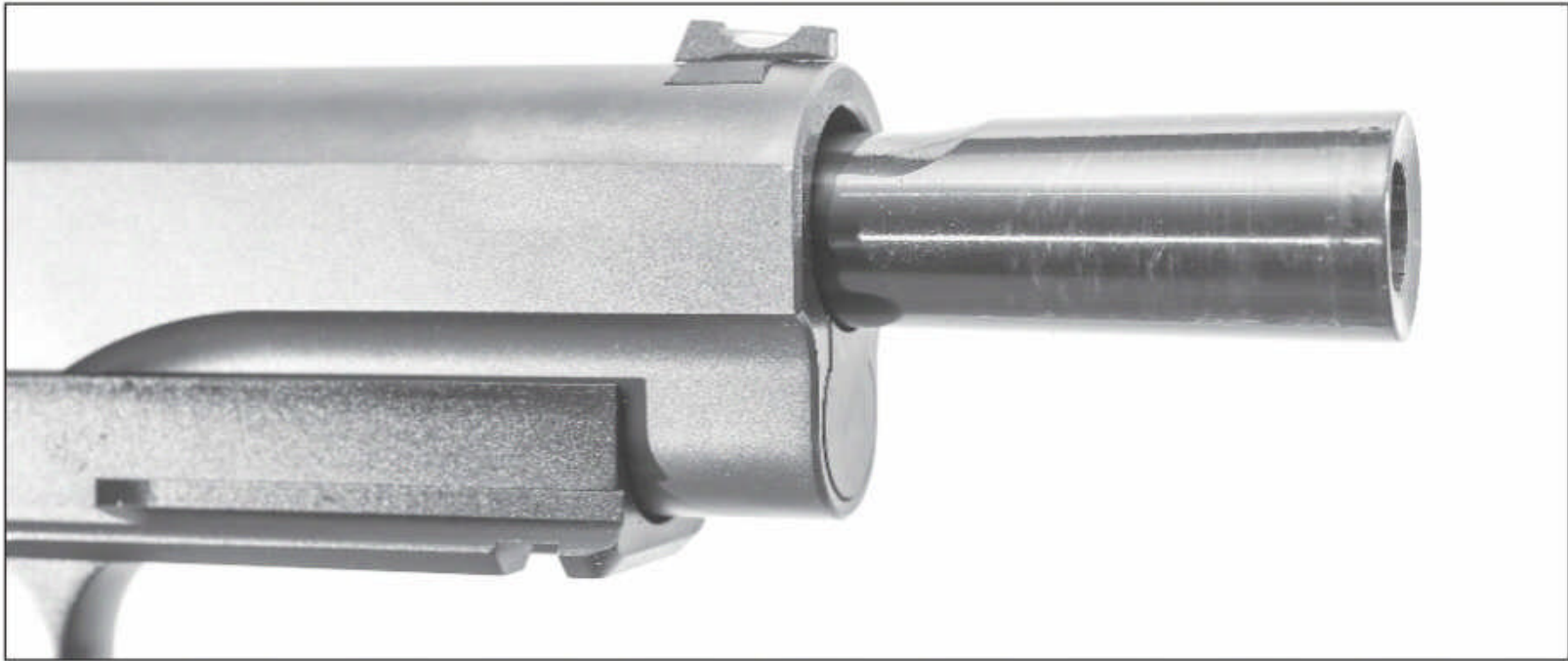
Here you can readily see the coned lockup of the Kodiak longslide barrel. No bushing, and no extra parts or machining for the bushing.
