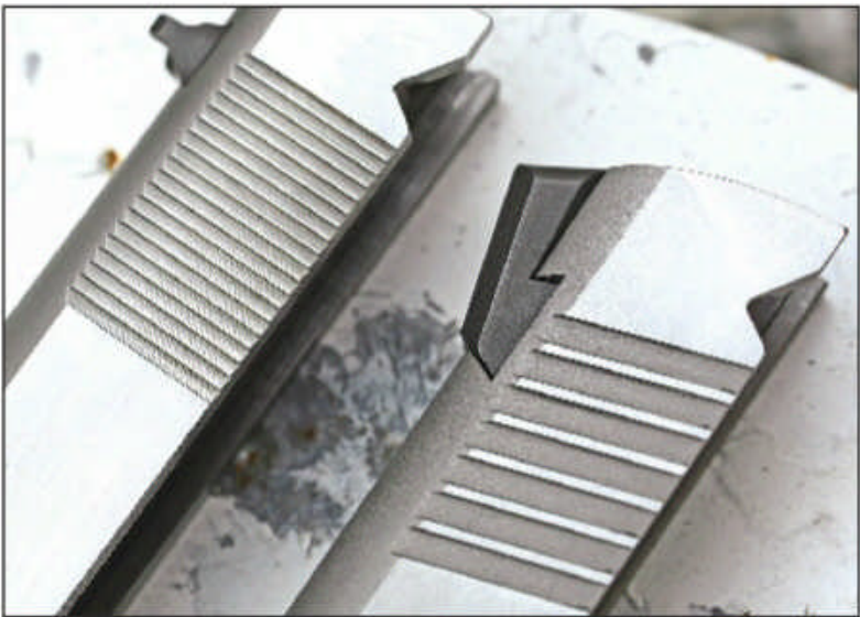
The old cocking serrations compared to the new, on the bottom.
