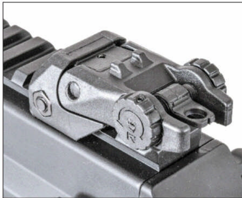
When folded the rear sight has two posts which work as a rear sight notch for use through the optic.
