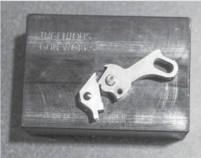
The Ingenious Gun Works hammer and sear would make Browning proud. They separate the safety drop notch from the sear engagement surfaces, and make the sear engagement a matter of geometry and not surface polishing.
