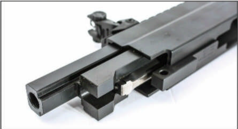
This is how the bolt fits into the receiver. No need for guide rods or rails, the bolt fits the receiver and is guided by it.
