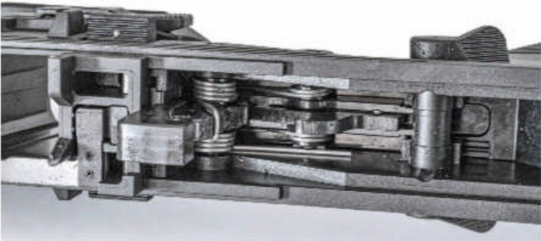
If the fire control group looks familiar, that's because the APC10 uses an AR-pattern hammer and trigger. Unlike an AR, you can engage the safety even if the hammer is not cocked.
