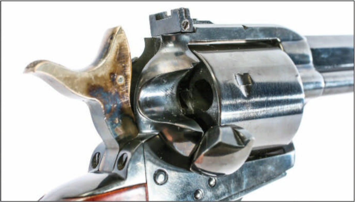
To load, cock the hammer to the first click, and flip open the loading gate. The cylinder will now spin freely, and you can load or unload.
