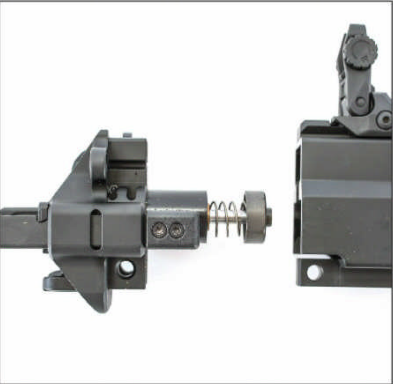
The stock assembly, showing the secondary buffer for the 10mm chambering. The APC10 needs it.
