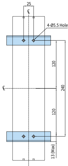
Mounting Drawing
