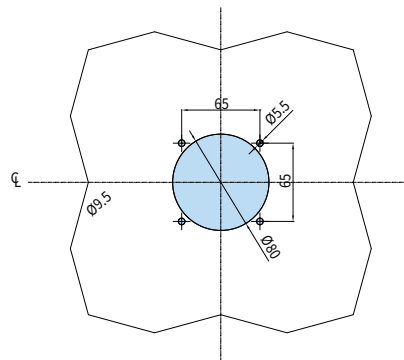
Extended Type
