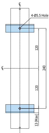
Mounting Drawing
