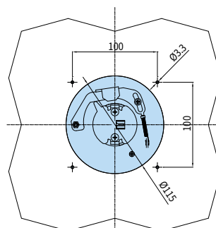
Extended Type
