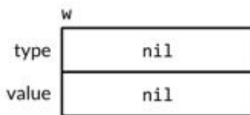
Figure 7.1. A nil interface value.
