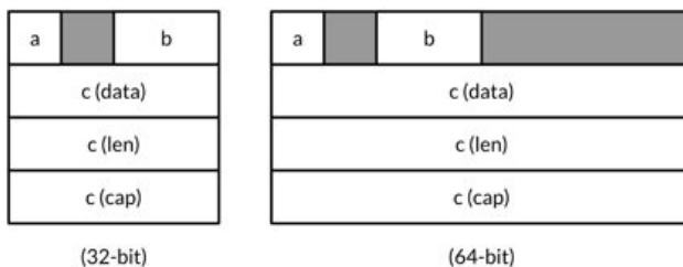
Figure 13.1. Holes in a struct.
