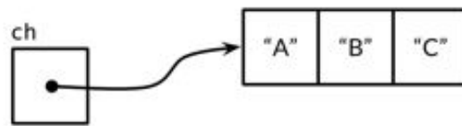
Figure 8.3. A full buffered channel.
