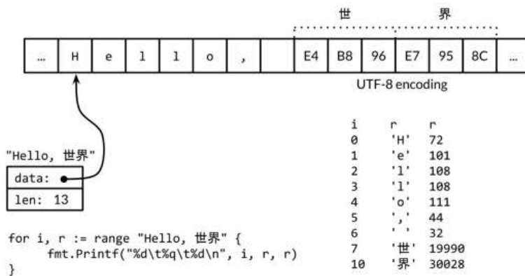
Figure 3.5. A range loop decodes a UTF-8-encoded string.
