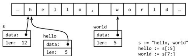
Figure 3.4. The string "hello, world" and two substrings.
