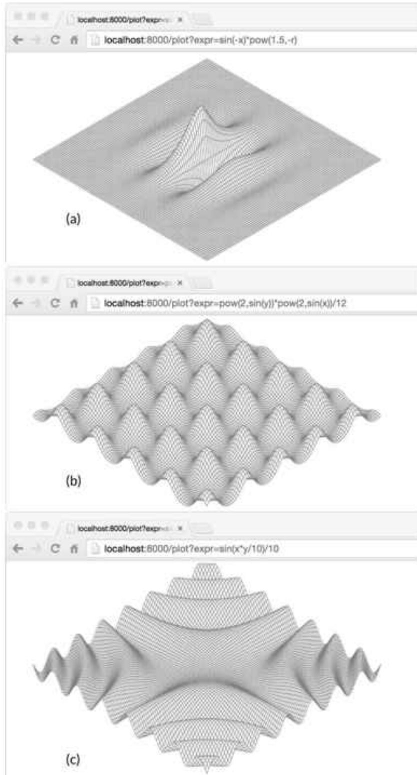
Figure 7.7. The surfaces of three functions: (a) \sin(-x) \cdot \text{pow}(1.5, -r) ; (b) \text{pow}(2, \sin(y)) \cdot \text{pow}(2, \sin(x)) / 12 ;
