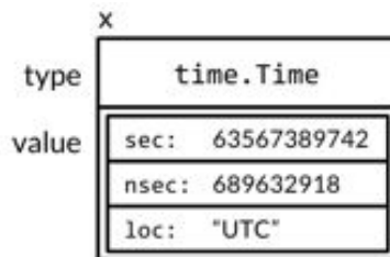
Figure 7.4. An interface value holding a time.Time struct.
