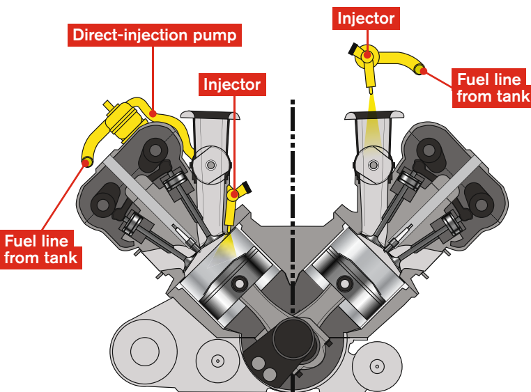
DIRECT INJECTION INDIRECT INJECTION
