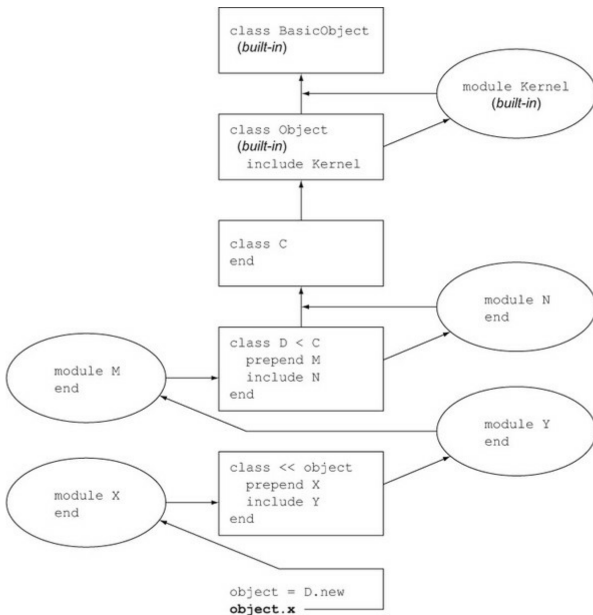
Figure 13.1. Method-search order, revised to include singleton classes
