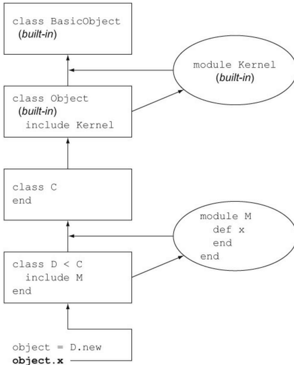
Figure 4.1. An instance of class D looks for method x in its method search path.
