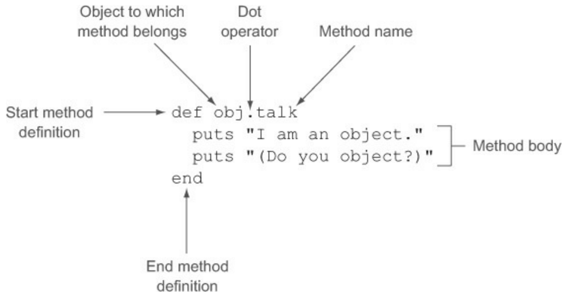
Figure 2.1. Anatomy of a method definition
