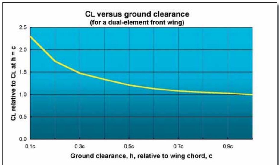
Figure 5: a generic plot, based on dual-element front wing data, of ground effect 'amplification' of downforce prior to viscous blockage at very small ground clearances (Competition Car Aerodynamics, McBeath)
