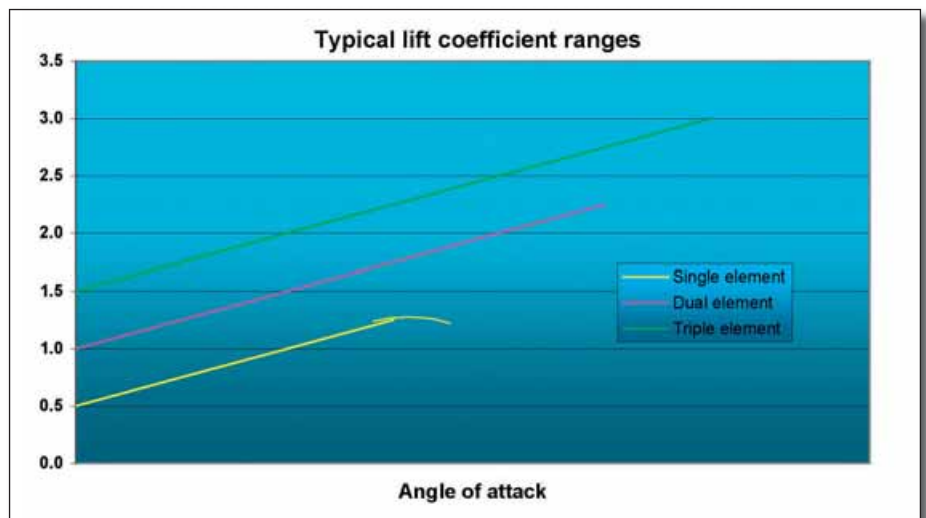
Figure 4: indication of the likely CL ranges for three basic wing configurations (McBeath)
