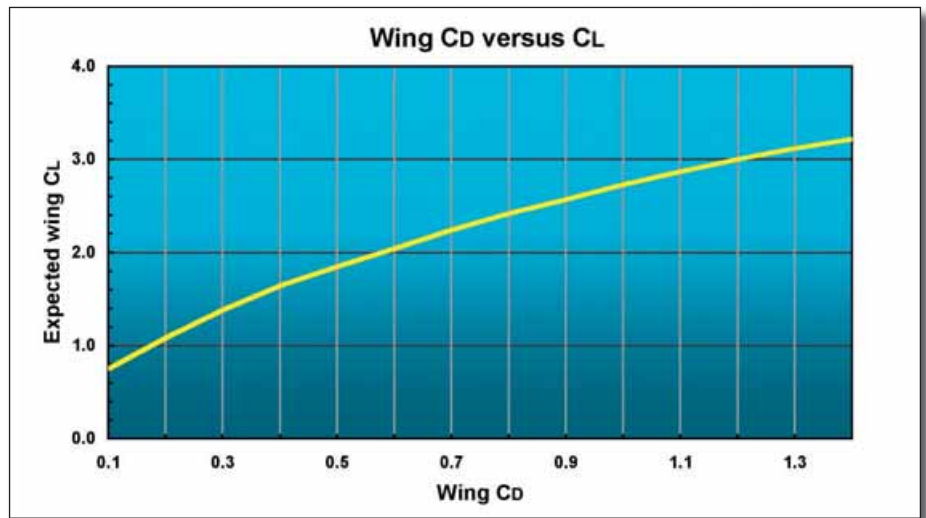
Figure 3: approximate correlation between wing CD and CL , based on published data on racecar wings (Competition Car Aerodynamics, McBeath)
