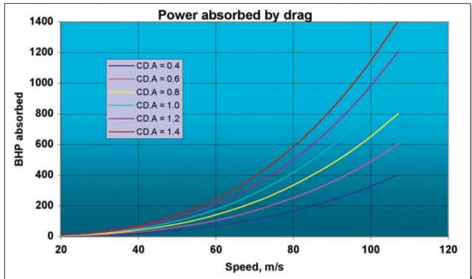
Figure 1: aerodynamic drag absorbs considerable power at higher racecar speeds (McBeath)
