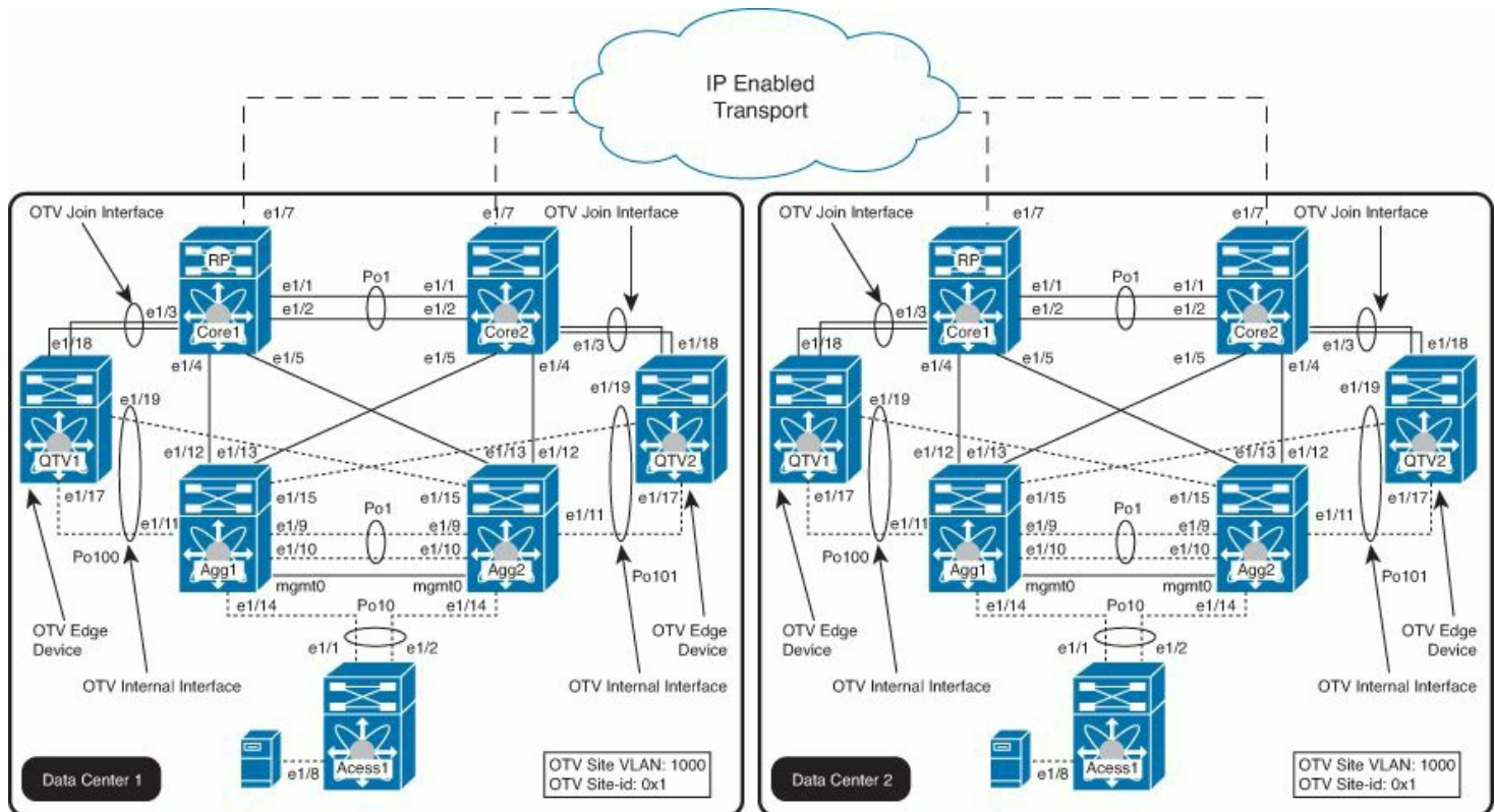
Figure 11-1. OTV Topology
