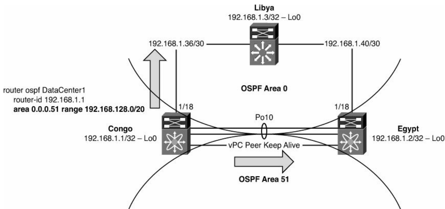
Figure 3-6. OSPF Summarization
