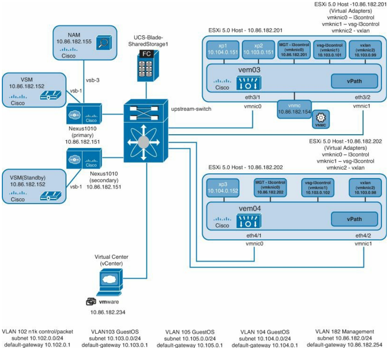
Figure 9-113. NAM Topology
