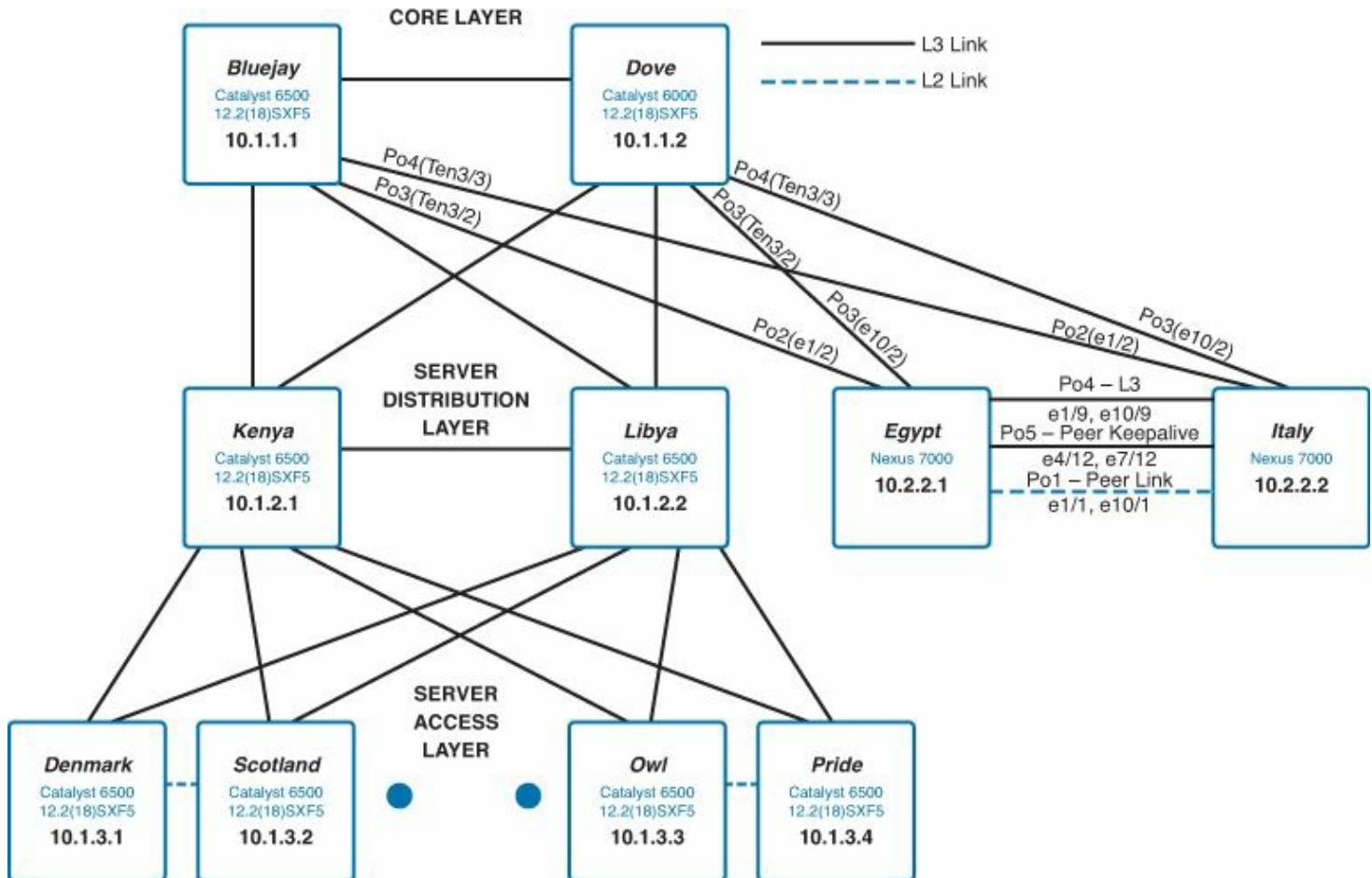
Figure 14-2. Current Topology
