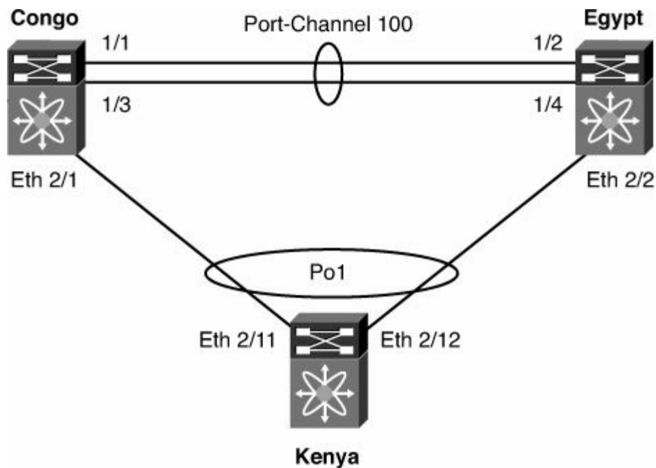
Figure 2-7. vPC Topology
