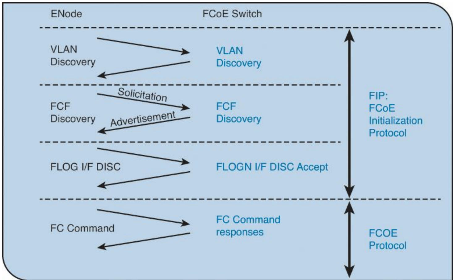
Figure 8-4. FIP Process
