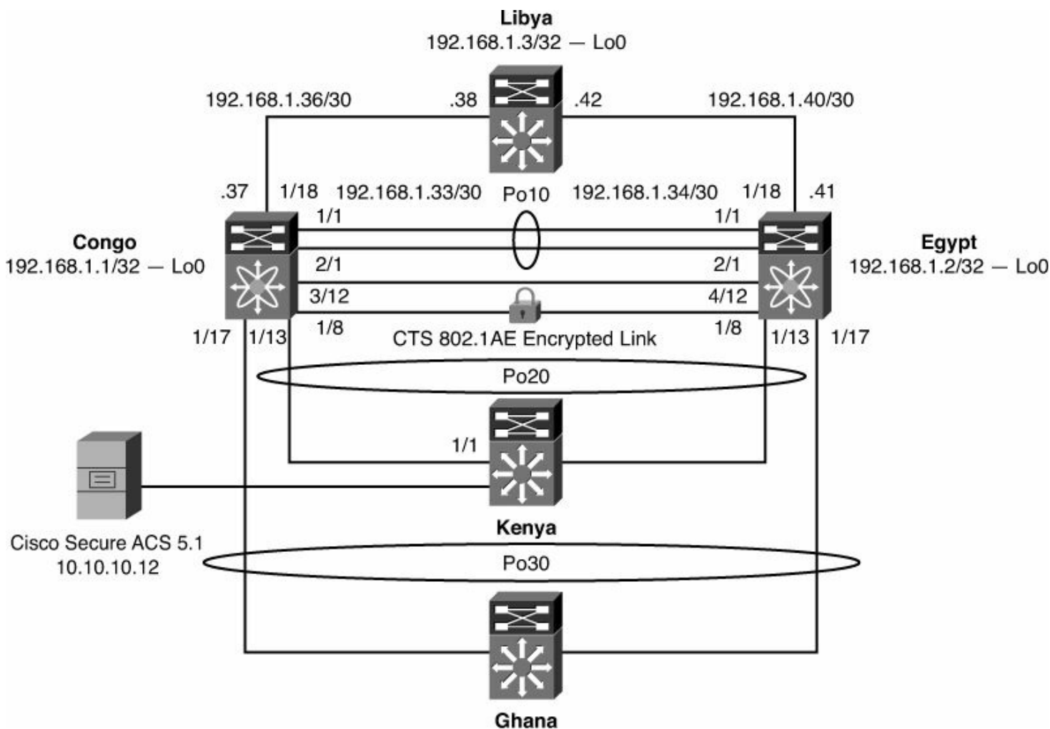
Figure 5-21. Cisco CTS 802.1AE Topology
