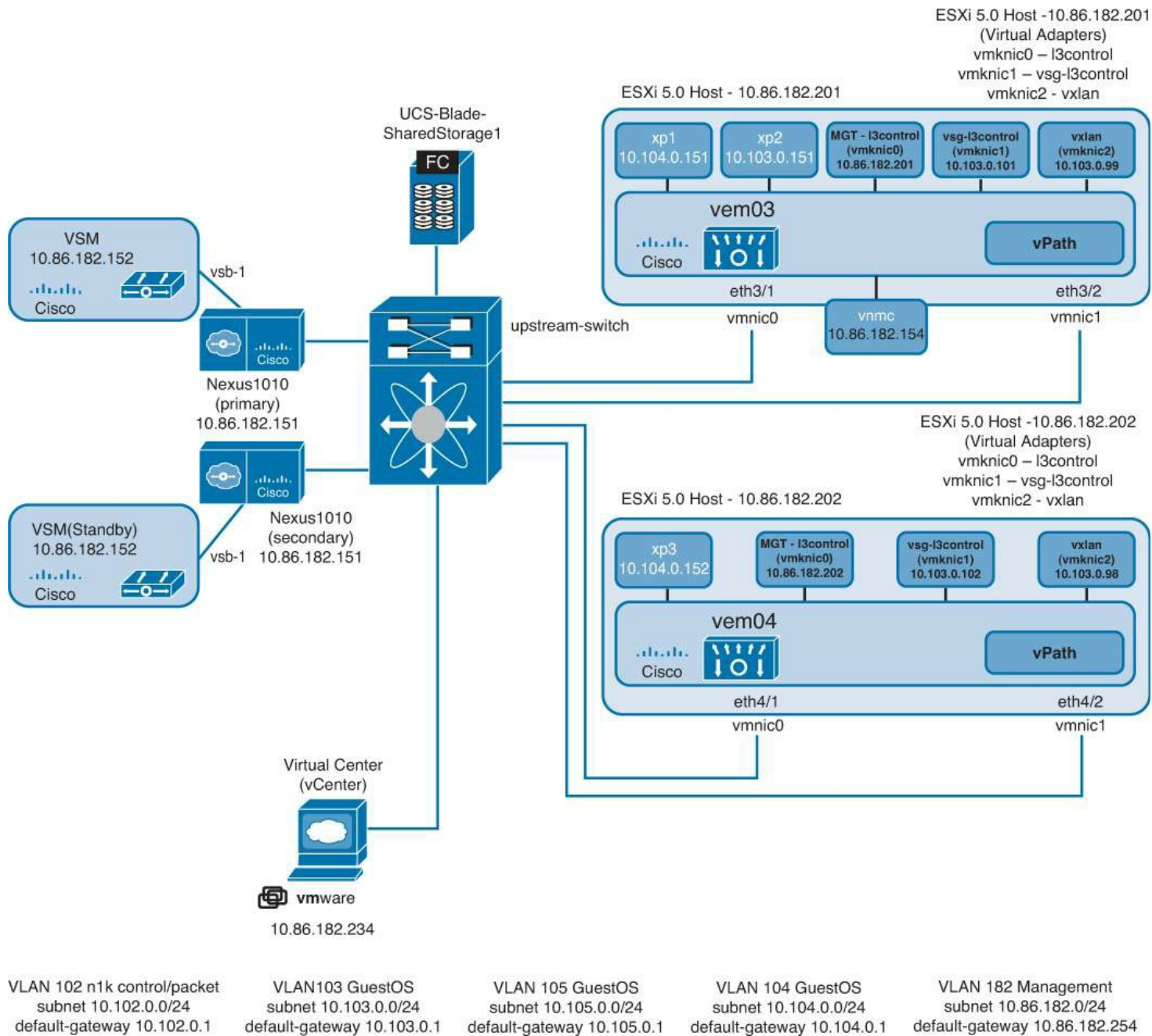
Figure 9-2. Nexus 1000V Topology
