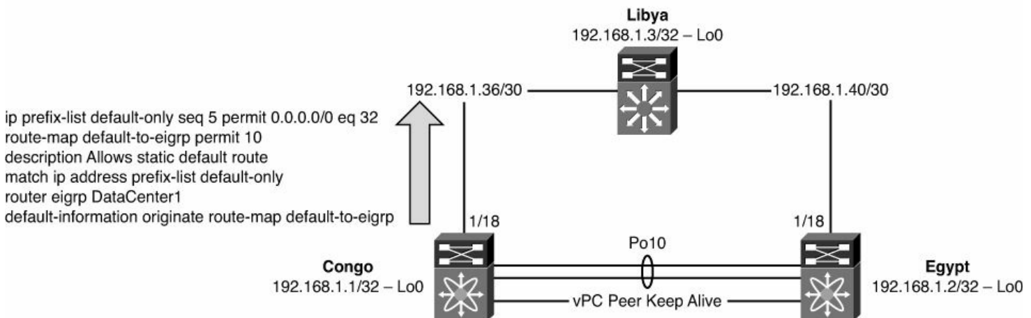
Figure 3-4. EIGRP Redistribution of the Default Route
