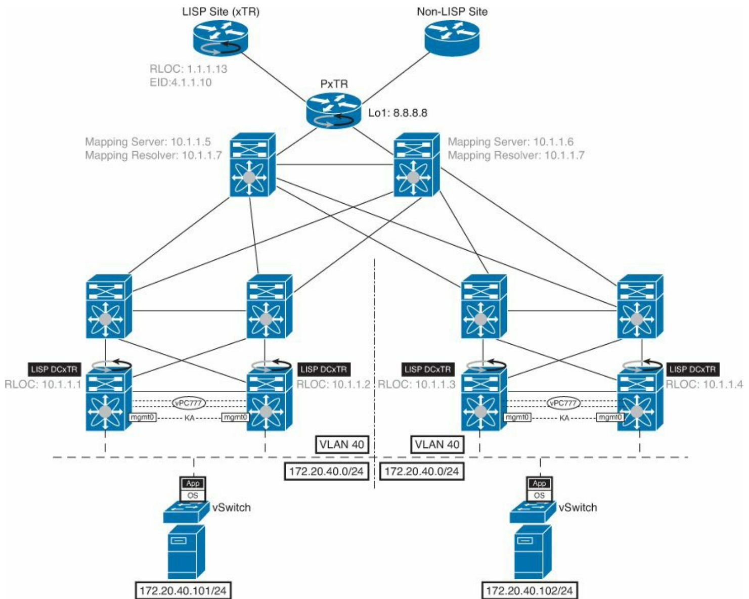
Figure 13-1. LISP Components
