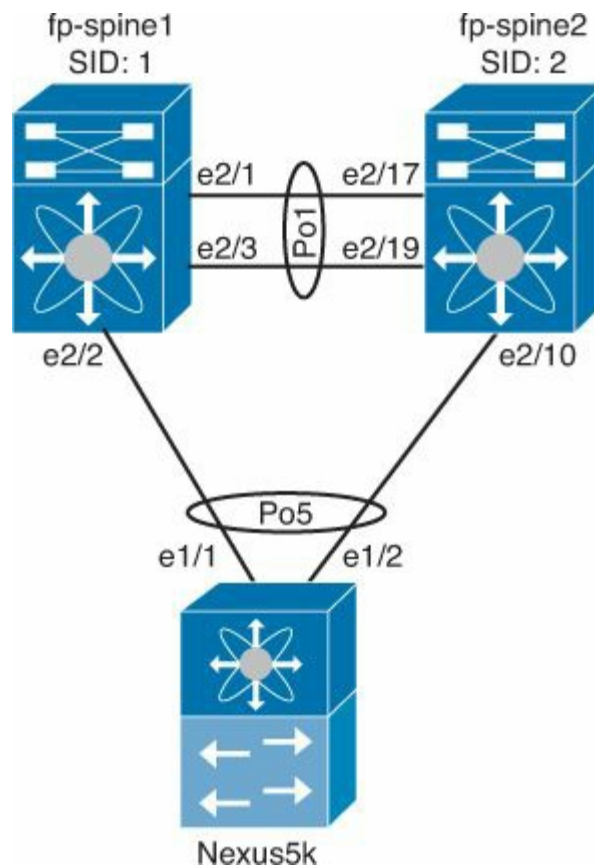
Figure 2-11. vPC+ Topology
