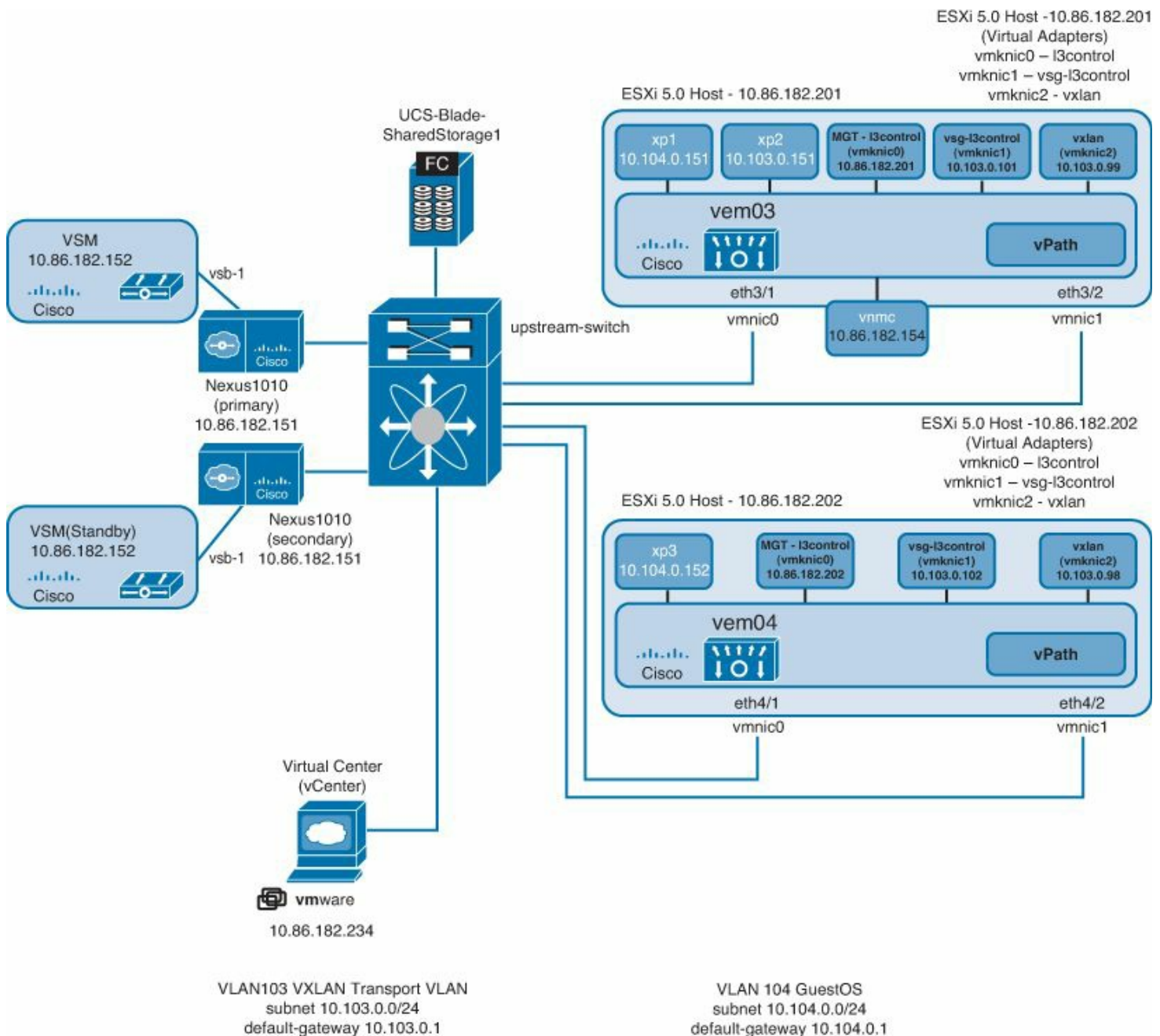
Figure 9-103. VXLAN Topology
