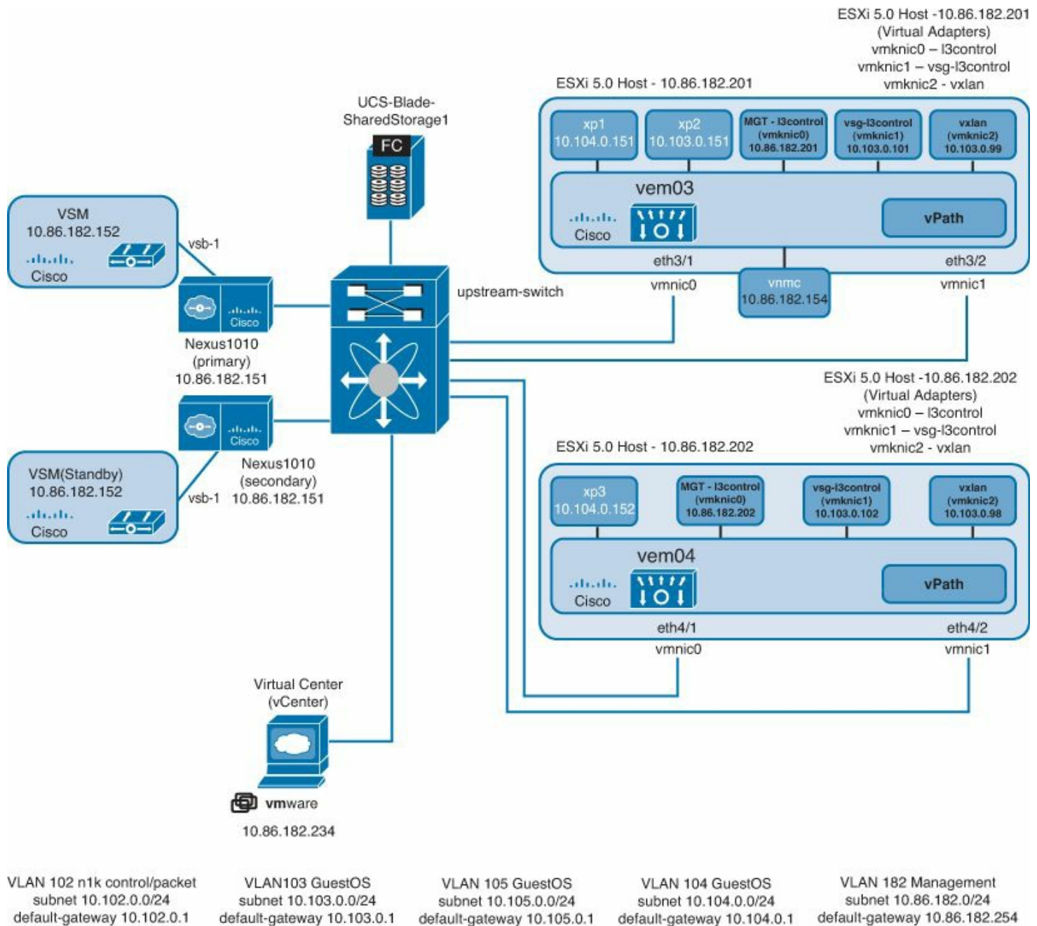
Figure 9-41. 1000V-Topology
