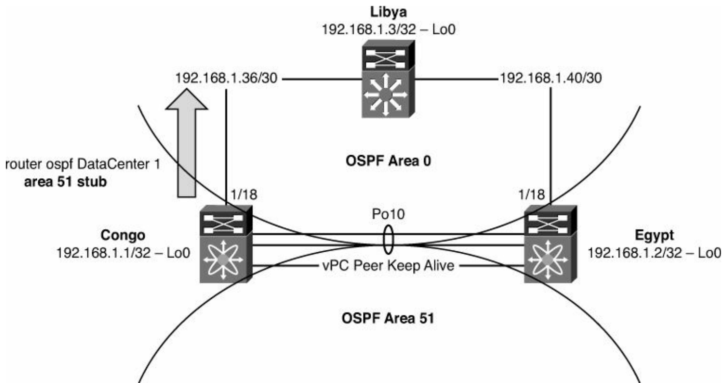
Figure 3-7. OSPF Stub
