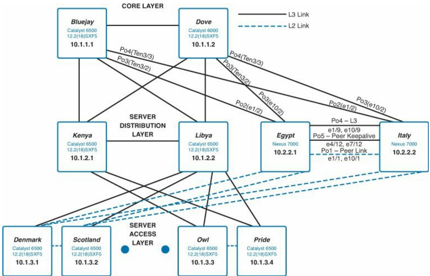
Figure 14-4. Migrated Topology
