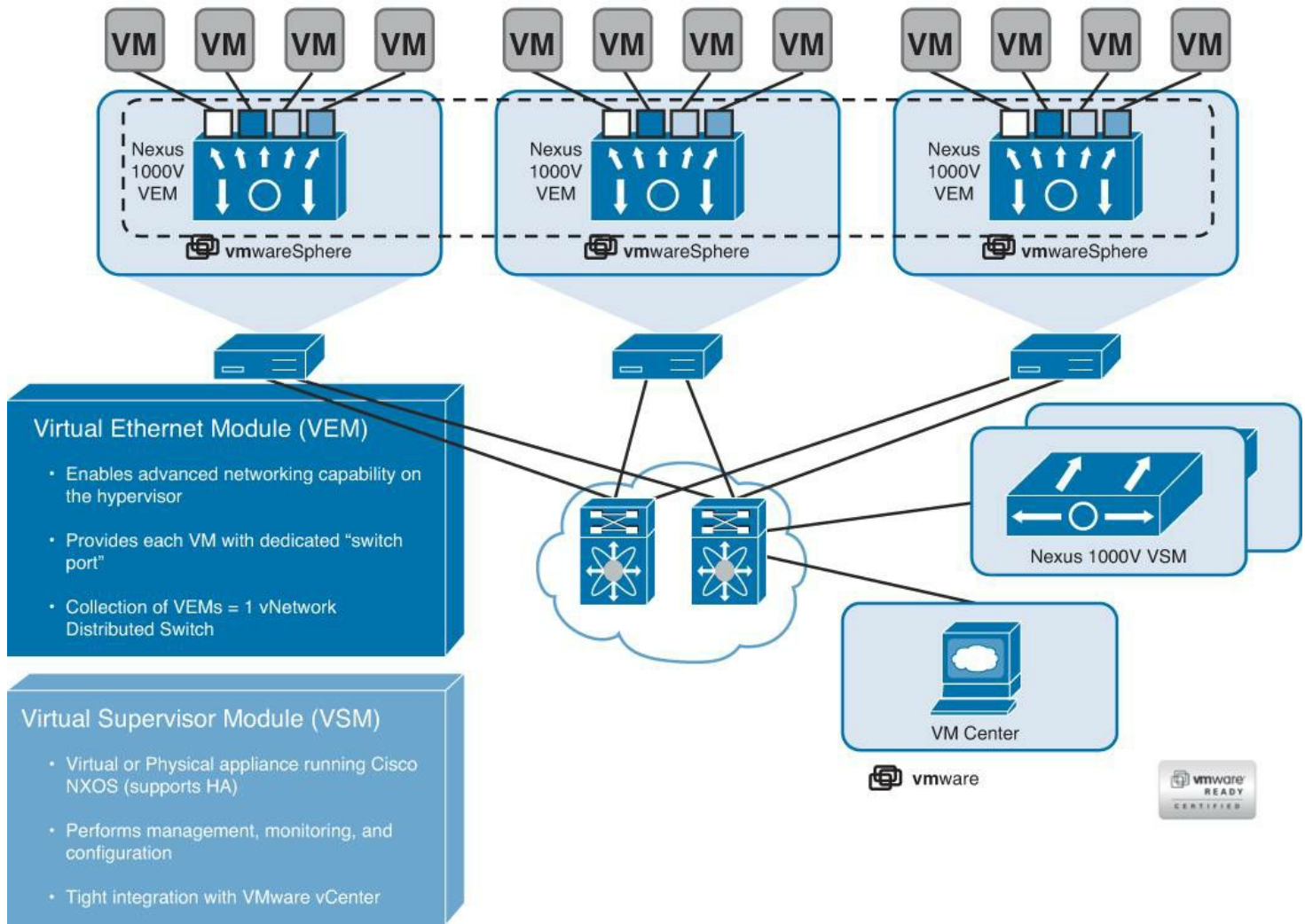
Figure 9-1. Cisco Nexus 1000V Series Architecture
