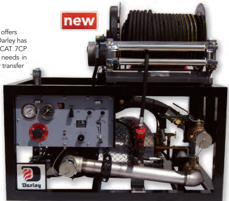
The UHP-HV® utilizes our patented Odin drive system driving our 2BE high volume pump and a high pressure CAT piston pump.
