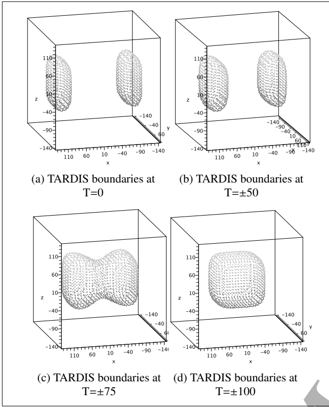
Figure 2: Evolution of the boundaries of the bubble, as defined in section II A, as seen by an external observer. At T = -100 the bubble will suddenly appear, and split in to two pieces which will move away from one another ( T = -75 , T = -50 ). At T = 0 , the two bubbles will come to rest, and then begin accelerating towards one-another ( T = +75 , T = +50 ). Whereupon, at T = +100 the two bubbles will merge and disappear.
