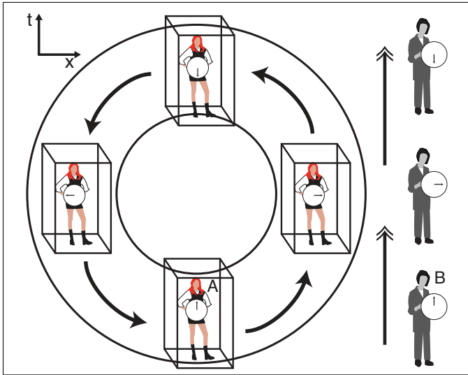
Figure 1: A schematic of the timelike observers confined to the interior and exterior of the bubble. Observers A (inside the bubble) and B (outside the bubble) experience the events in dramatically different ways. Arrows indicate the local arrow of time . Within the bubble, A will see the B's events periodically evolve, and then reverse. Outside the bubble, observer B will see two versions of A emerge from the same location: one's clock hands will turn clockwise, the other counterclockwise. The two versions of A will then accelerate towards one another and annihilate.
