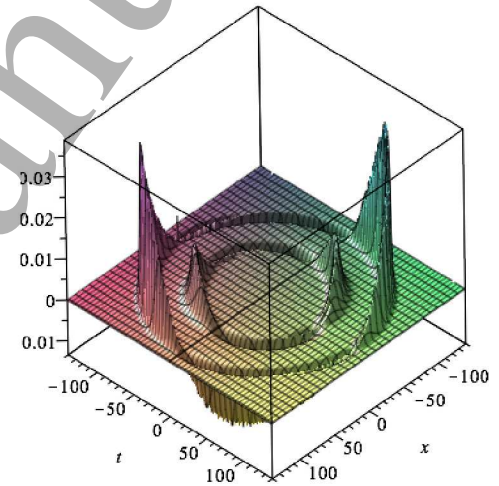
(b) The value G_{ab}N^aN^b along z = 1 , y = 1 , where N^a is a null vector field along the surface.
