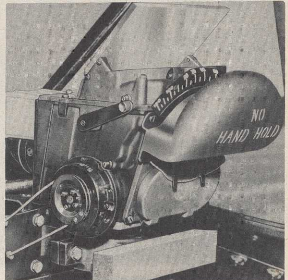
LIGHT RHEOSTAT AND SIGHT SELECTOR OF K-14 GUNSIGHT ARE ON THE LEFT SIDE OF COCKPIT.
