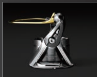
Redesigned Magnumlite Rotor now has the bail arm mechanism on the opposite side to the line roller for improved balance and lighter overall weight.
