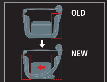
Redesigned Magnumlite Rotor now has the bail arm mechanism on the opposite side to the line roller for improved balance and lighter overall weight.
