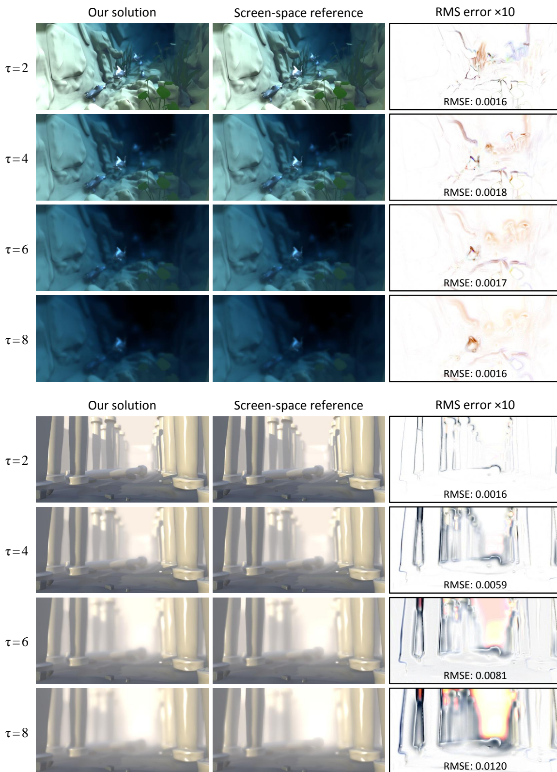
Figure 3.4: Evaluation of SSS for different values of medium optical thickness \tau in a highly absorbing underwater environment ( top ) and a high-albedo fog ( bottom ). Numerical evaluation against the screen-space reference is included to gauge the performance of our filtering solution under different optical conditions.
