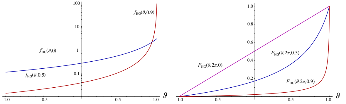
Figure 5.6: Plots of f_{HG} (left) and F_{HG} (right) for parameter g values of 0, 0.5 and 0.9. Please note that the plots of f_{HG} have a logarithmic scale and the values of F_{HG} are evaluated for the full azimuthal range, i. e., |\phi_1 - \phi_2| = 2\pi .
