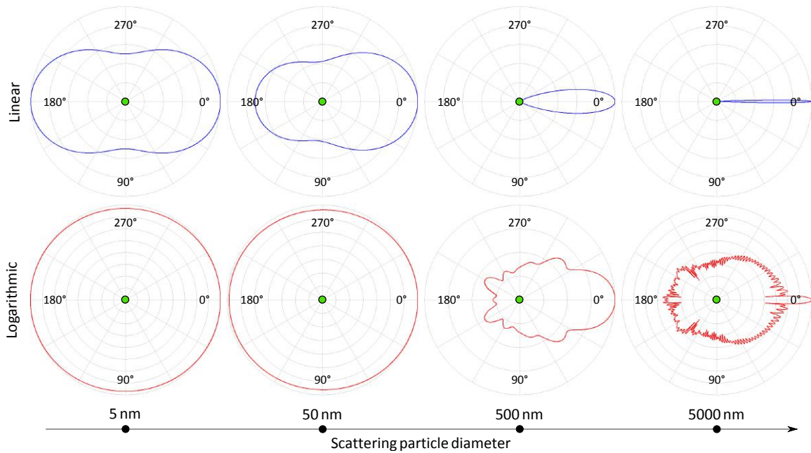
Figure 2.4: Plots of Mie phase functions for several orders of scattering particle sizes (computed for \lambda = 500 \text{ nm} ). For small particles in the order of single nm, the phase function converges to the Rayleigh approximation ( left ). Generated with MiePlot (Philip Laven, http://www.philiplaven.com/mieplot.htm ).
