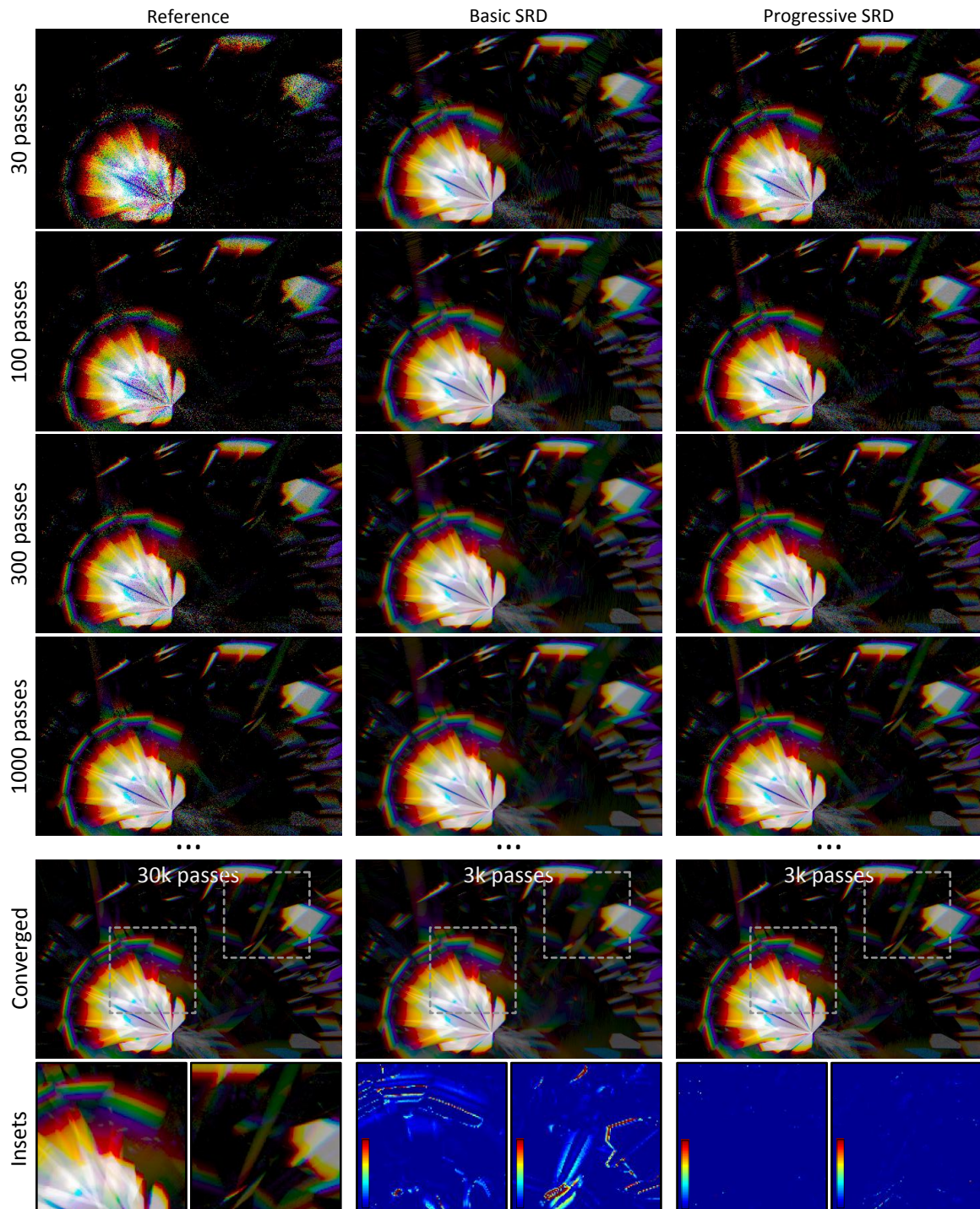
Figure 6.13: Progressive convergence of the “diamond” caustic (see Section 6.6.2 for a detailed discussion). The insets show false-colour-coded RMSE differences between the SRD / PSRD solutions and the reference.
