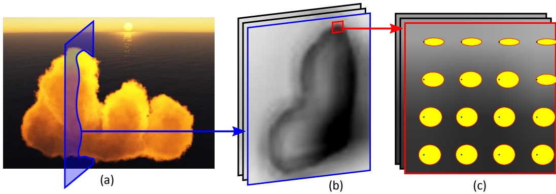
Figure 4.7: Local Henyey-Greenstein lobes – (b) shows a slice of the greyscale-encoded anisotropy coefficients of the illumination solution that correspond to the marked region in the cloud (a). The exact shape of the lobes in the cache locations is shown in (c). The light in (c) is coming from the left.
