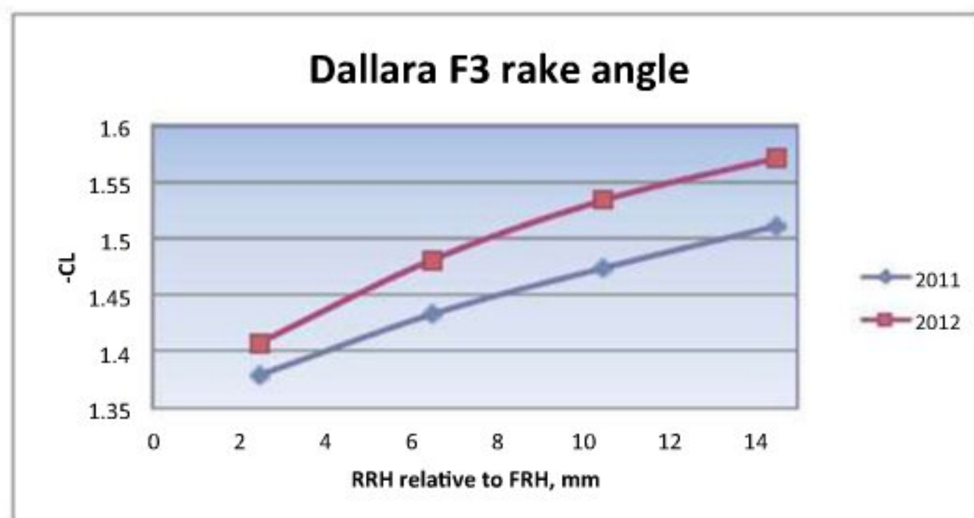
Figure 1: the effect on -CL, overall lift coefficient, of changing rake angle
