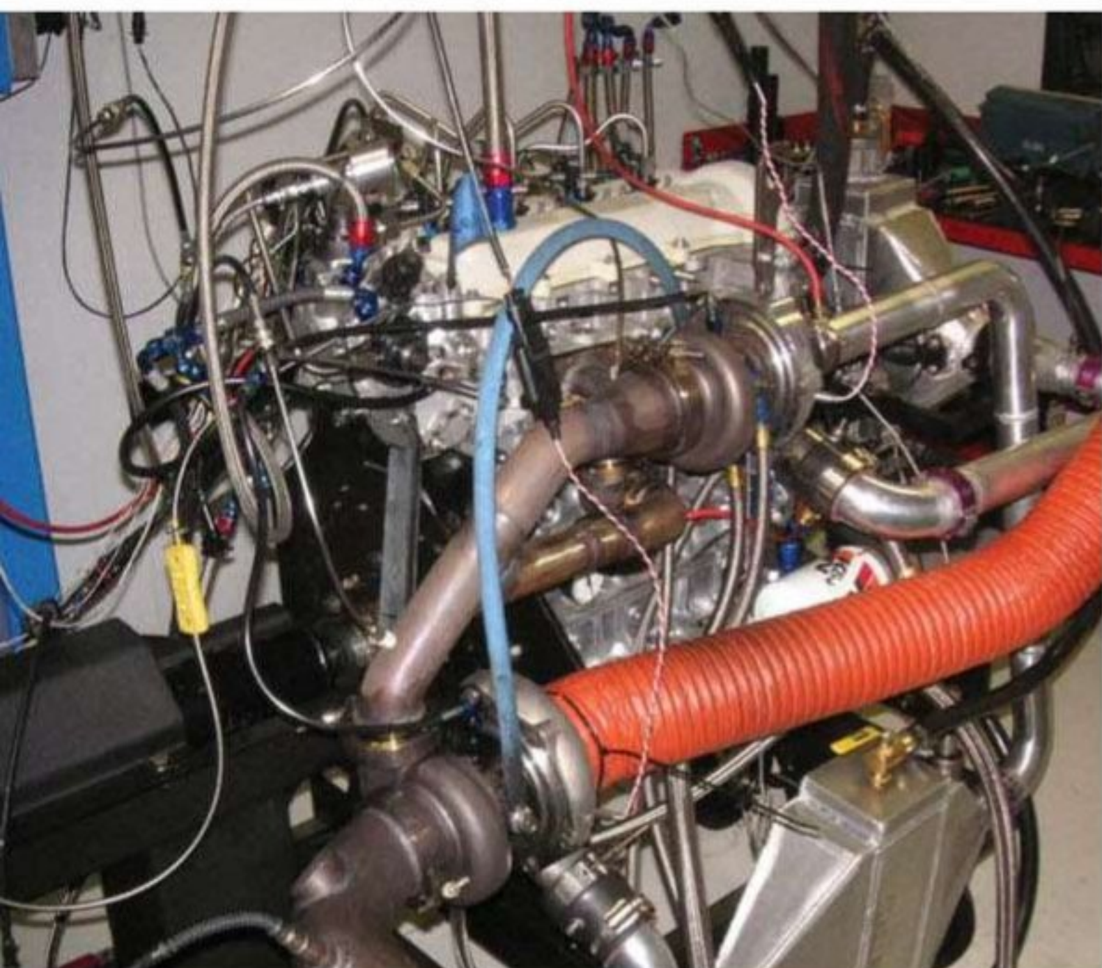
Though much of the production engine's components are up to the job in terms of strength, the race versions will use bespoke internals for improved durability
