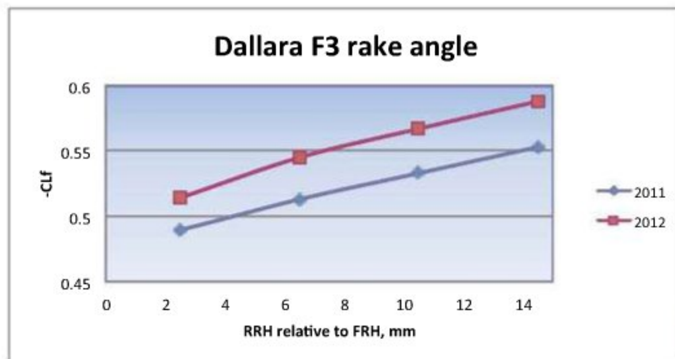
Figure 2: the effect on -CLf, front lift coefficient, of changing rake angle
