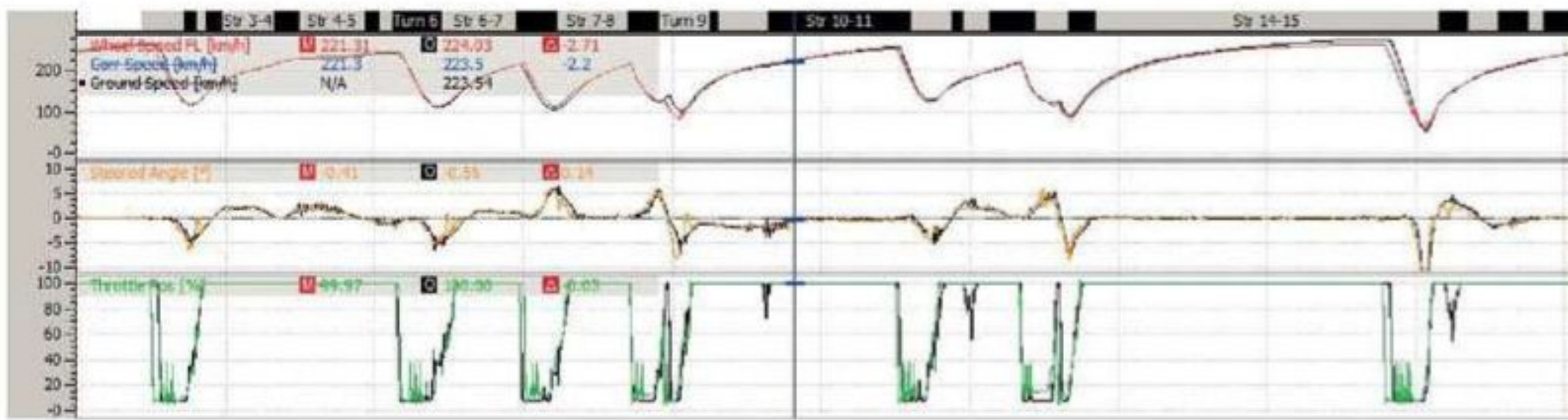
Figure 3: initial correlation
