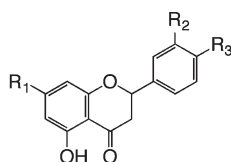
Figure 2. Flavone- C -glucosides ( 1 , 2 ) and flavone- O -glycosides ( 6 ). † O -Neohesperidose.
