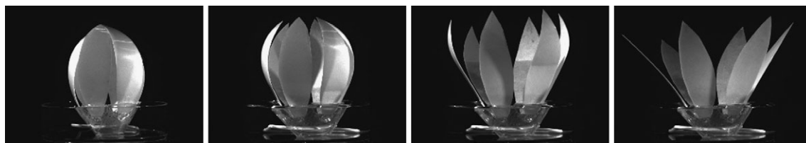
Figure 5. A floral mimic made of paper–plastic bilayer petals shows a controllable blooming and wilting response. When dipped in water, the petals open and the flower blooms, while when the water supply is exhausted, the bilayer dries out and the flower closes (see electronic supplementary material, movies S6 and S7). The length of the petals is about 4 cm, and the typical time scale of a cycle is an hour.
