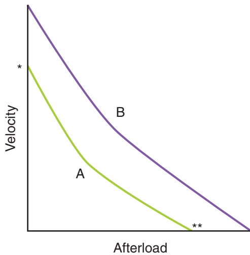
Figure III-2-2. Force–Velocity Curve
