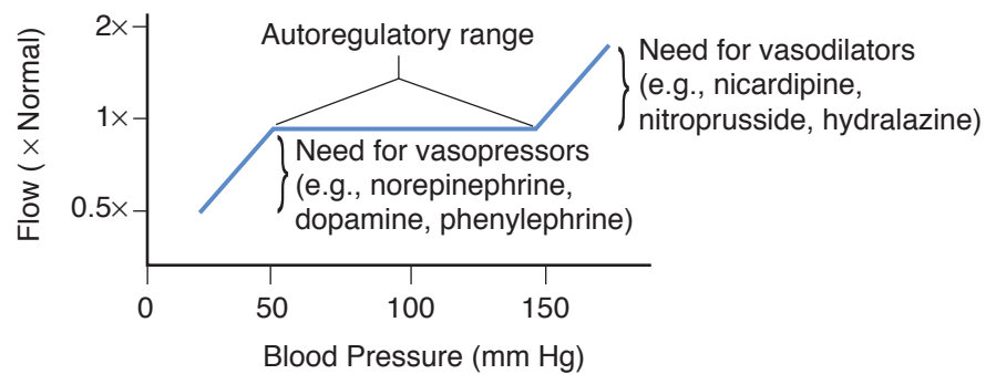
Figure V-2-3. Autoregulation
