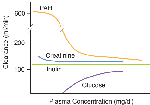
Figure VIII-3-2. Clearance Curves
