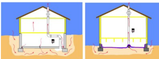
Active Soil Depressurization
