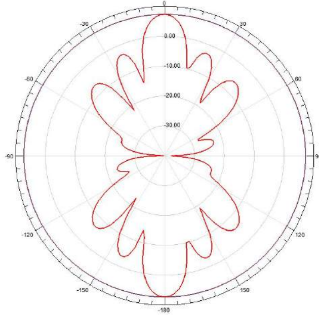
H Plane
