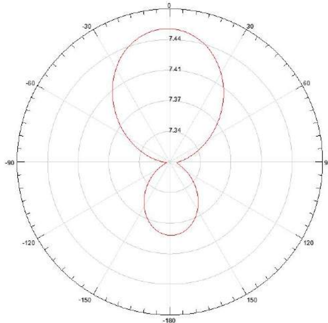
E Plane
