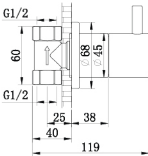
SC103-05 -25mm (FT)
