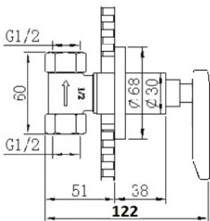
SC102D-03 -20mm (QT)
