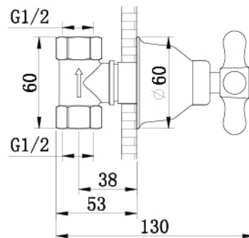
SC102D-04 -20mm (QT)
