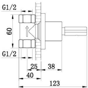
SC102D-07 -20mm (QT)
