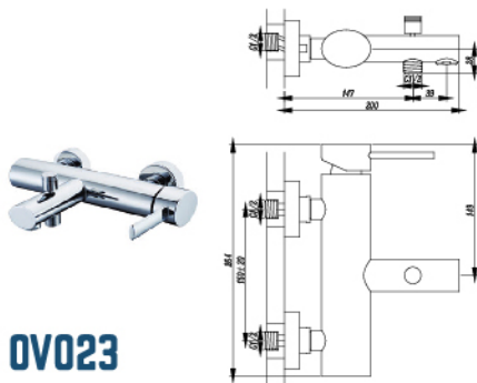
Exposed Bath & Shower Mixer
