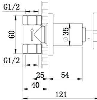
SC102D-06 -20mm (QT)
