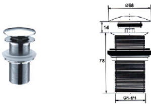
I6504 SPRING WASTE WITHOUT OVERFLOW RM 75.00
