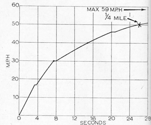
ACCELERATION GRAPH
