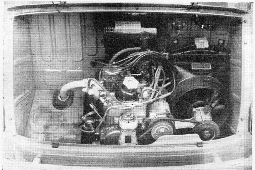
STOWAWAY: (Above) Packed away in the rear boot, as if by an afterthought, is the very willing little 633 c.c. four-cylinder o.h.v. engine and its auxiliaries.
