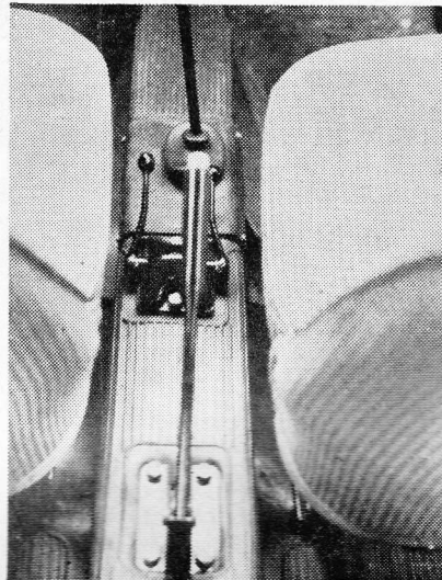
ALL IN A ROW: Positioned between the seats, on top of the control tunnel, are the gear lever, choke and starting controls and the handbrake.
