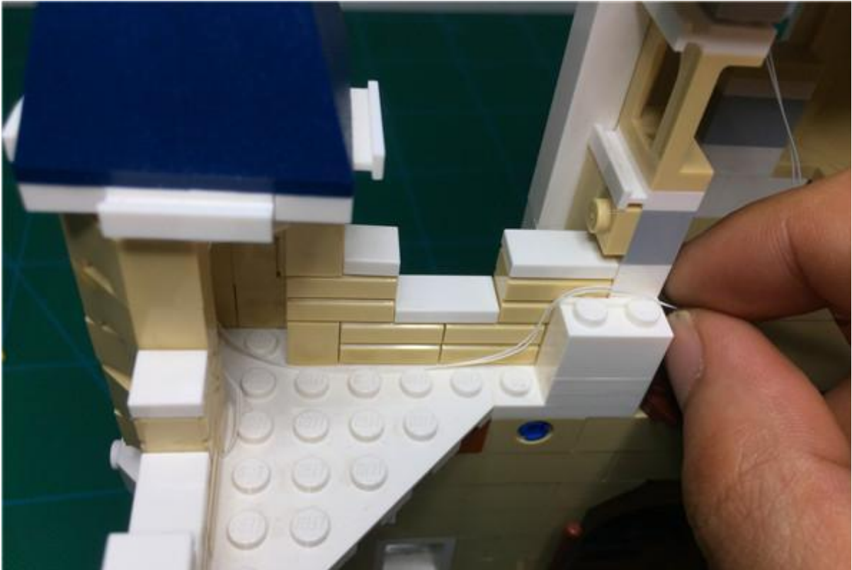
Along to the wall and into the white part
