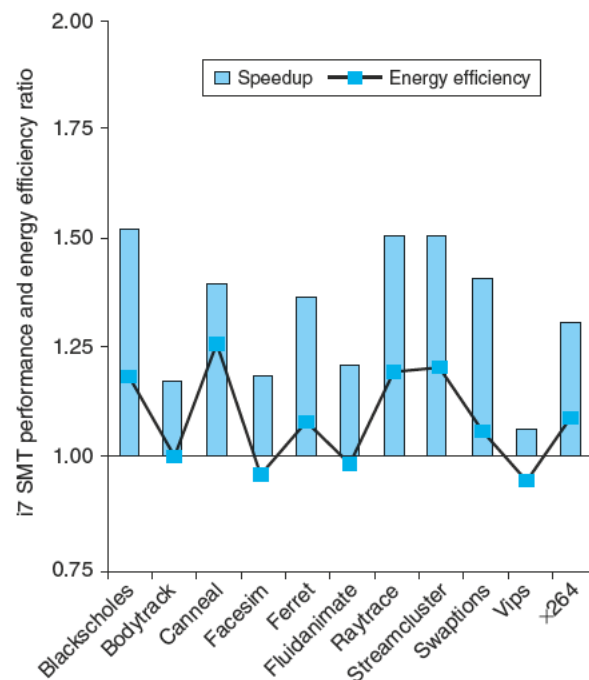
FIGURE 6.6 The speed-up from using multithreading on one core on an 17 processor averages 1.31 for the PARSEC benchmarks (see Section 6.9 ) and the energy efficiency improvement is 1.07 . This data was collected and analyzed by Esmaeilzadeh et. al. [2011].
