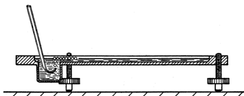
FIGURE 1. Apparatus for producing rafts of bubbles.
