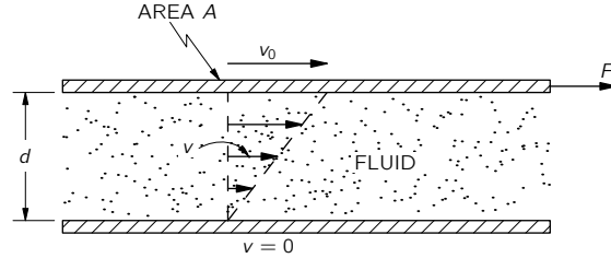
Fig. 41-1. Viscous drag between two parallel plates.
