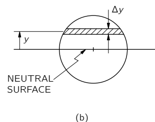
Fig. 38-12. (a) Small segment of a bent beam. (b) Cross section of the beam.
