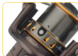
Rubber-buffered and spring-loaded Safety Line Clip PLUS and spool with hole to fix the line reliably with line stoppers
