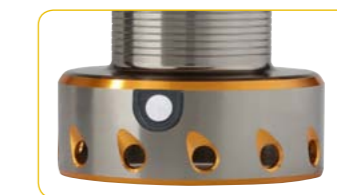
Rubber-buffered Safety Line Clip and spool with hole to fix the line reliably with special line stoppers
