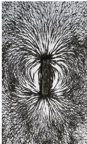
MAGNETIC FIELD
