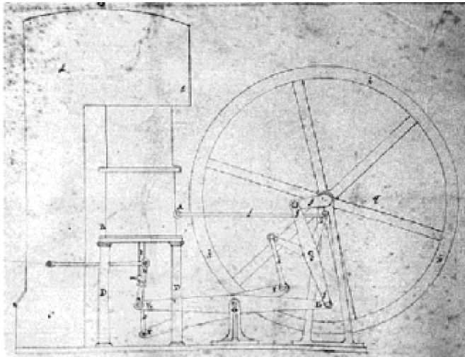
Stirling generator Patent Design Plans.
