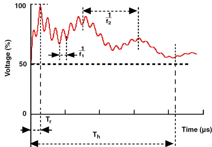
Figure 3—Typical very fast front short-duration overvoltages ( T_r = 3\text{--}100\text{ ns} , T_h < 3\text{ ms} , f_1 = 0.3\text{--}100\text{ MHz} , f_2 = 30\text{--}300\text{ kHz} where T_r is the time-to-crest, T_h is the time-to-half value, f_1 and f_2 are the frequencies of the superimposed oscillation; f_1 and f_2 are defined in the figure)
