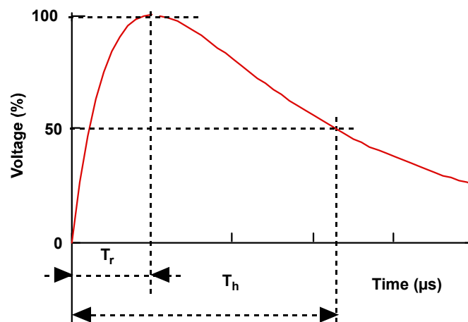
Figure 2—Switching overvoltages ( T_r = 20\text{--}5000 \mu\text{s} , T_h < 20\,000 \mu\text{s} , where T_r is the time-to-crest value, T_h is the time-to-half value)
