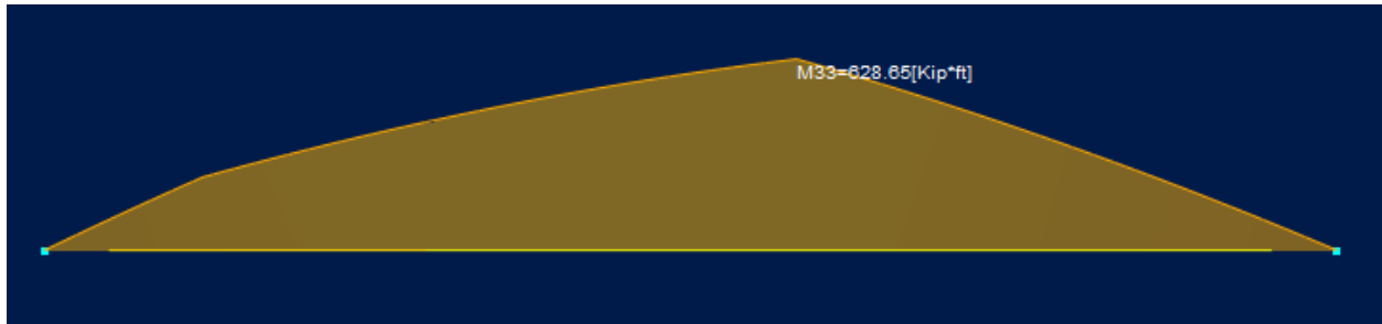
Unfactored Moment (self-weight + 20 psf construction load)
