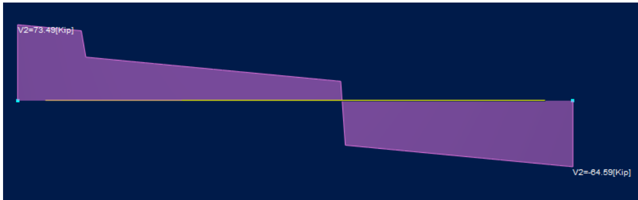
Unfactored Shear (self-weight + 20 psf construction load)
