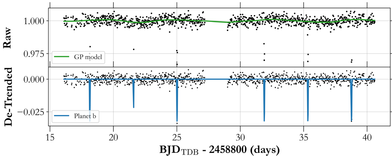
Figure 1. Long-cadence (30 minute) time-series TESS eleanor photometry from Sector 19, along with a stellar rotation GP kernel ( RotationTerm from celerite2 ) in green. The detrended photometry is shown in the bottom panel, with the TOI-3757 b transits overlaid in blue.
