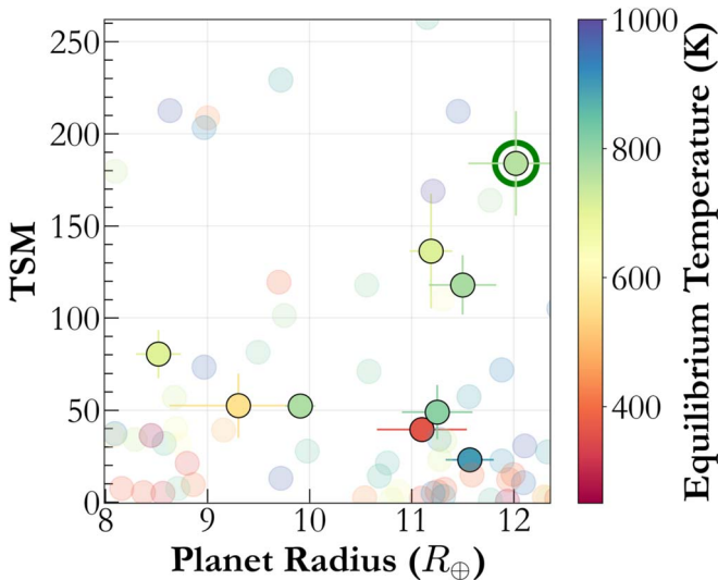
Figure 11. TSM of TOI-3757 b (circled in green) as a function of the planetary radius, alongside other M dwarf Saturn- and Jupiter-type planets ( R_p > 6 R_{\oplus} ; colored by the equilibrium temperature). Similar planets around FGK hosts with equilibrium temperatures < 1000 K are shown in the background. TOI-3757 b has the highest TSM among M dwarf gas giants ( R_p > 6 R_{\oplus} ) with mass measurements, making it a lucrative target for atmospheric characterization, as discussed in Section 5.2.
