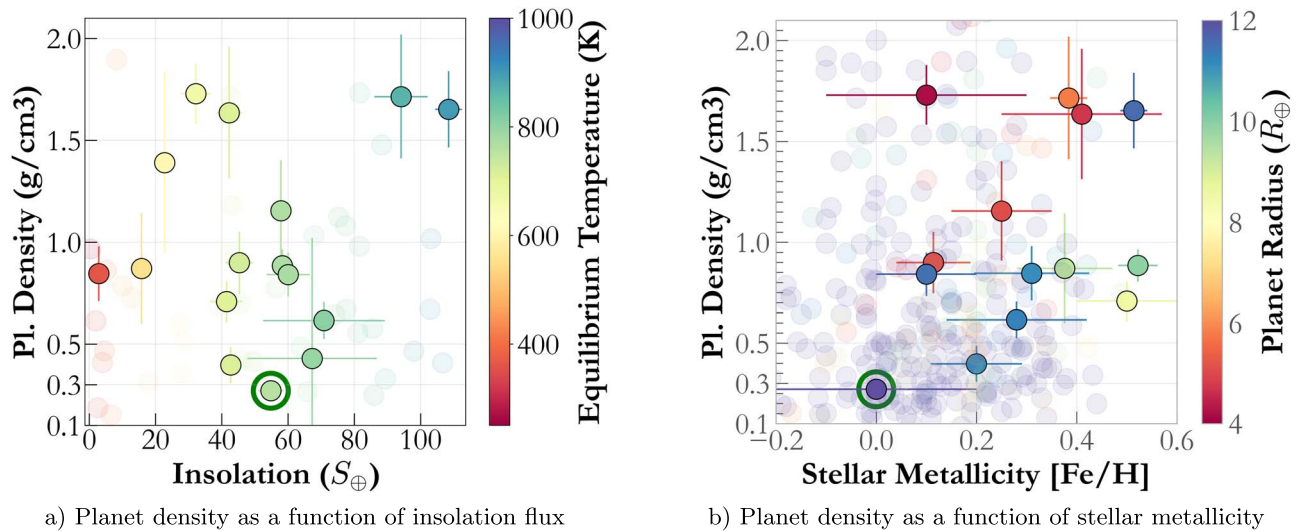
Figure 10. We show the planetary density of gas giants ( R_p > 4 R_\oplus ) around M dwarfs (solid colors) as a function of stellar insolation and stellar metallicity, respectively. In panel (a) the markers are color coded by the equilibrium temperature, whereas panel (b) is color coded by planetary radius. Additionally, TOI-3757 b is highlighted with a green circle. In panel (a), we show that TOI-3757 b does not receive an unusually large amount of incident flux from its host star, compared to other similar gas giants. In panel (b), we show that the host star has the lowest metallicity of all known gas giants around M dwarfs, which could be a potential explanation of its density.
