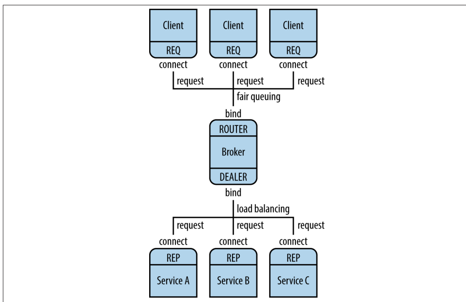
Figure 11-1. Using a broker to connect multiple clients and services
