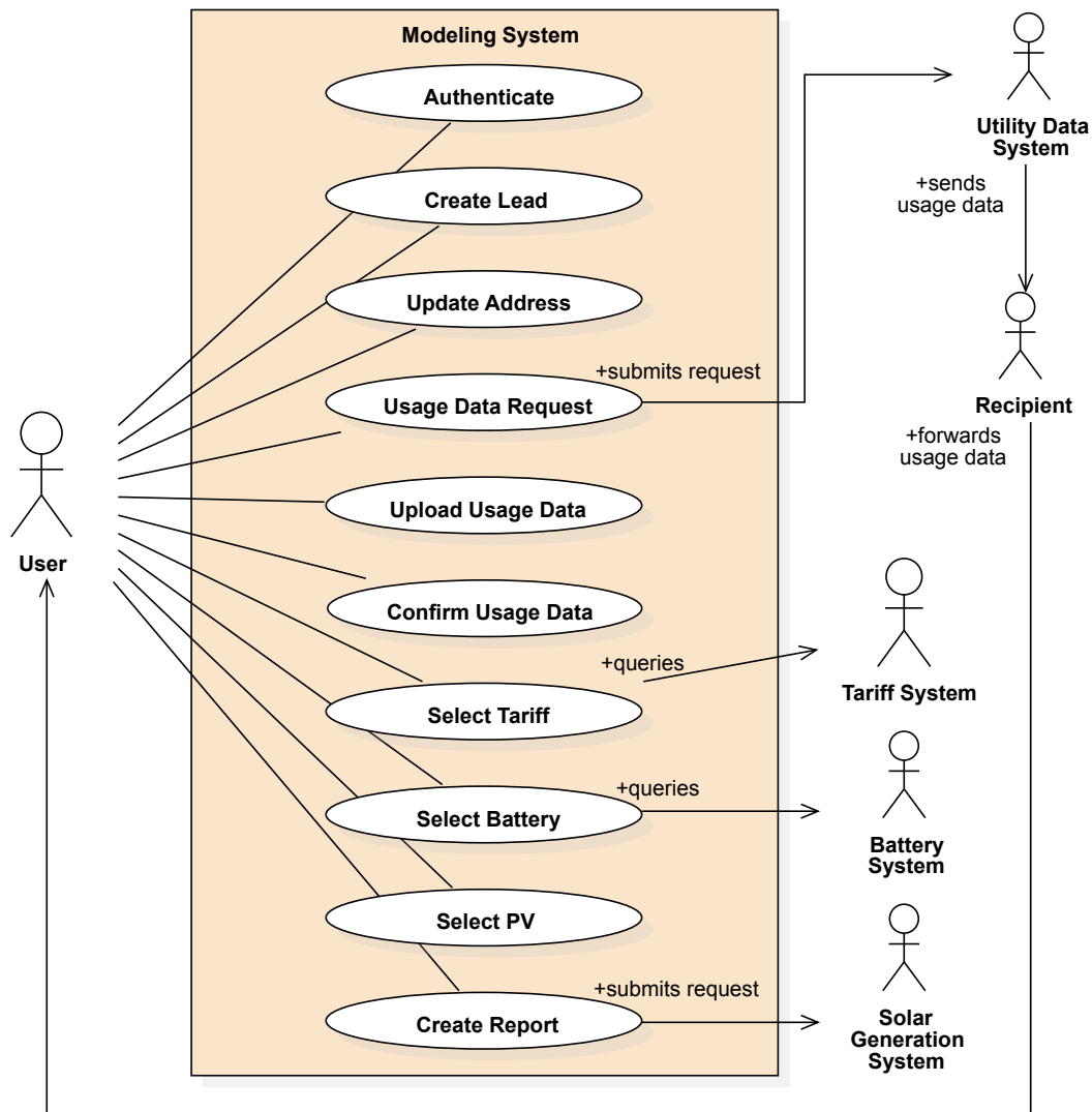
Figure 4.1 Use Case 001
