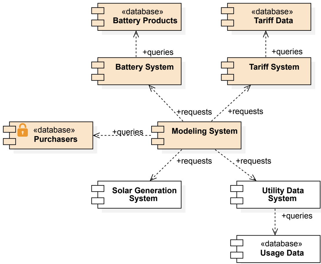
Figure 3.1 Architectural Components
