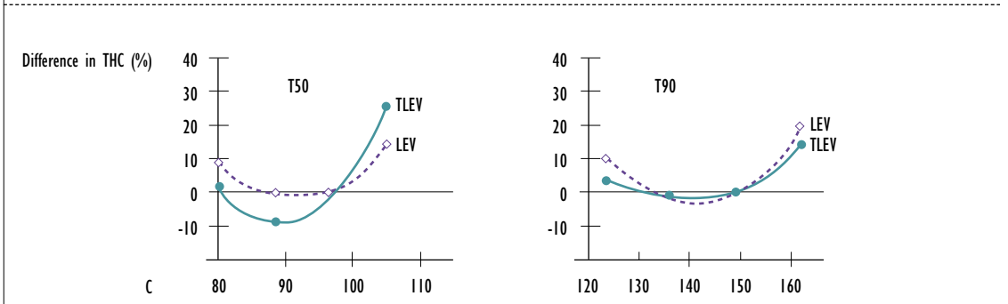
Figure 22: Effect of T50/T90 on Exhaust Emissions Comparison of LEV and TLEV
