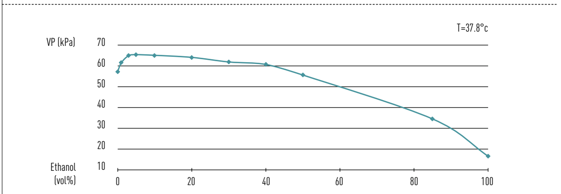
Figure 23: Impact of Ethanol Level on Vapour Pressure at 37.8 °C
