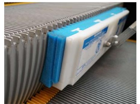
Cleaning vertical part using Sponge Pad
