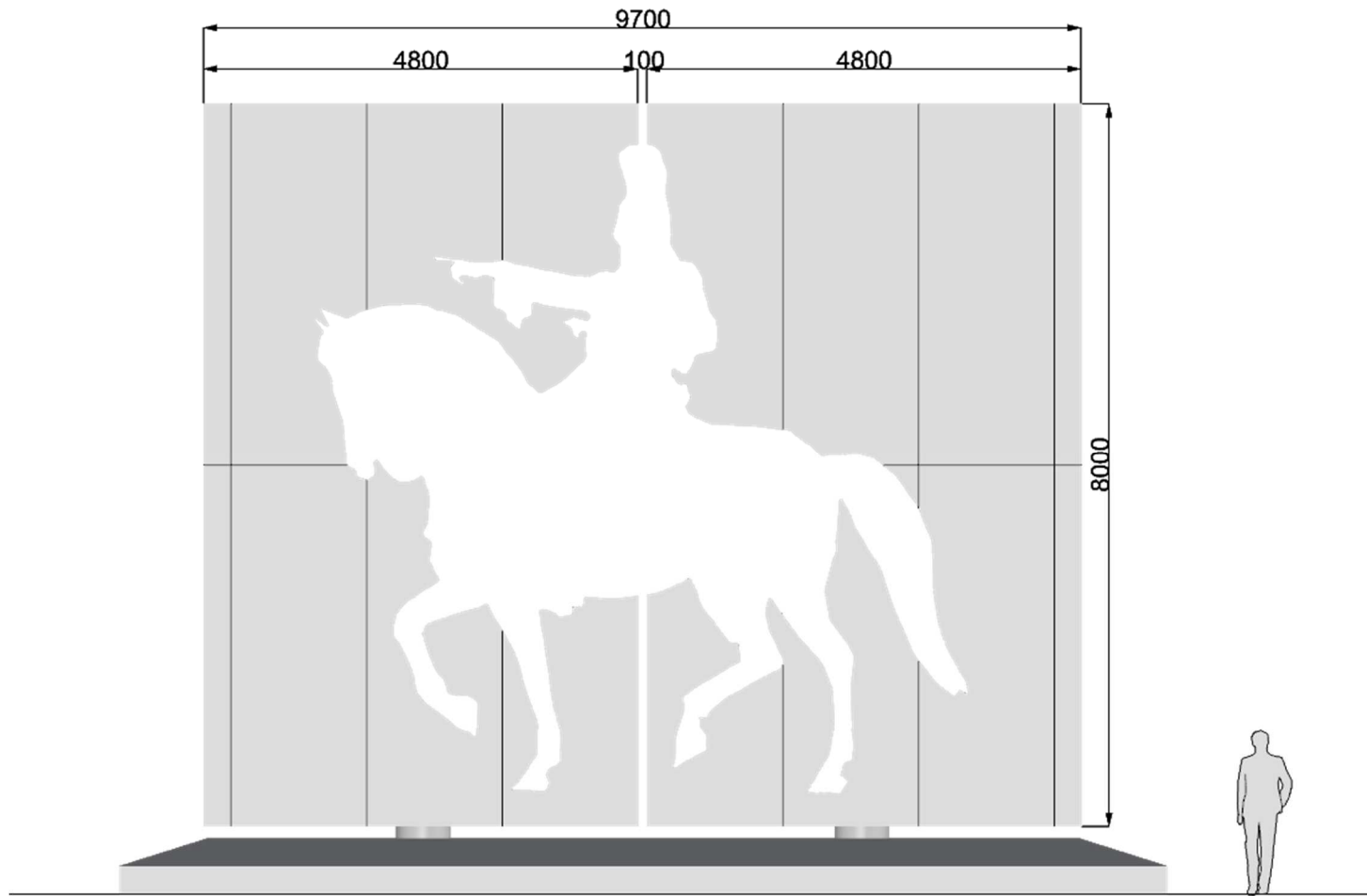
OVERALL DIMENSIONS OF THE SCULPTURE (MM)
