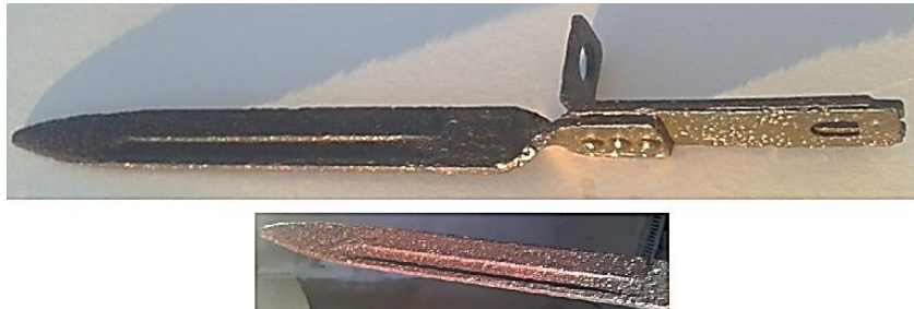
Rare variety of M95 twist blade. Represents only about 0.3% of all Austrian ersatz bayonets. It has different grip stave design and fullered blade. The blade is longer, 260mm wide and about 6-7mm thick. This example is in relic condition and is missing a blade tip.
