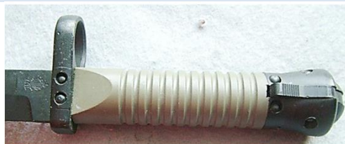
Air Force of the CETME L bayonet. It features a distinctive hilt catch similar to the G3 types
