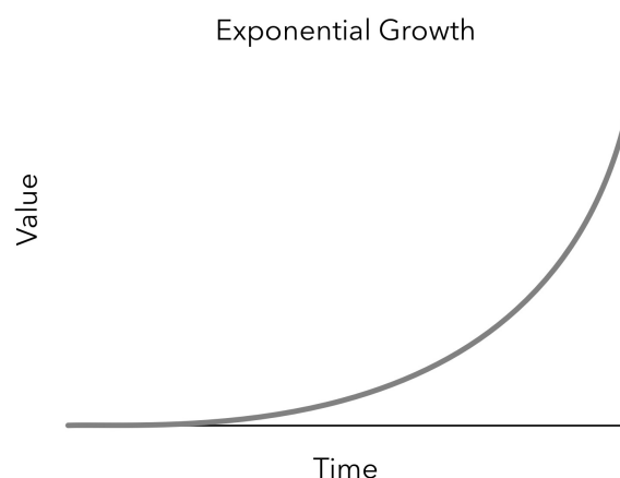
Figure 1: An exponential growth curve due to compounding.
