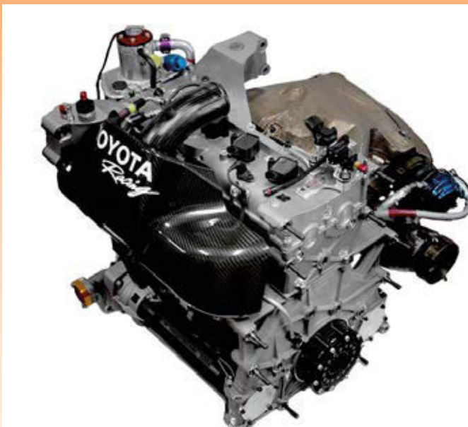
GT500 in Japan initially ran with 3.4-litre V8s but, for 2014, GTA rules demand 2.0-litre turbocharged four cylinder powerplants like this Lexus unit
