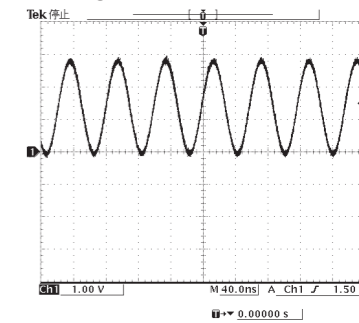
POINT ⑤ XL501 (Pin 109 of IC503)
