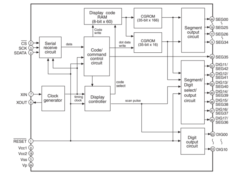
IC801: M66003-0131FP-R 18 digit 5 x 7 segment VFD controller/driver
