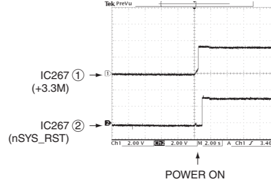
POINT ① IC267 (99 pin, +3.3M), ② IC267 (12 pin, nSYS_RST)
