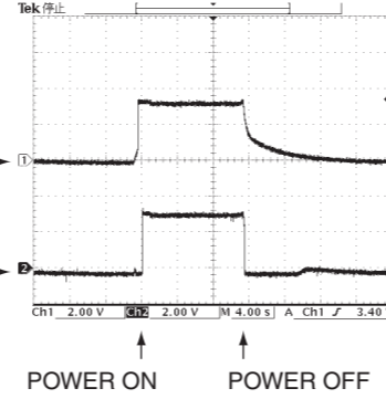
POINT ① IC267 (99 pin, +3.3M), ② IC267 (12 pin, nSYS_RST)
