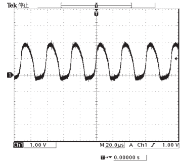
POINT ③ XL253 (Pin 11 of IC267)
