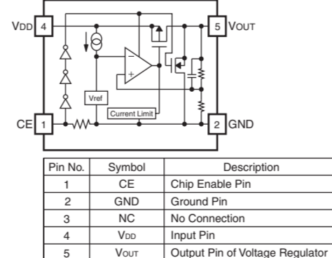
IC902: R1172H121D-T1-F CMOS-based positive-voltage regulator IC
