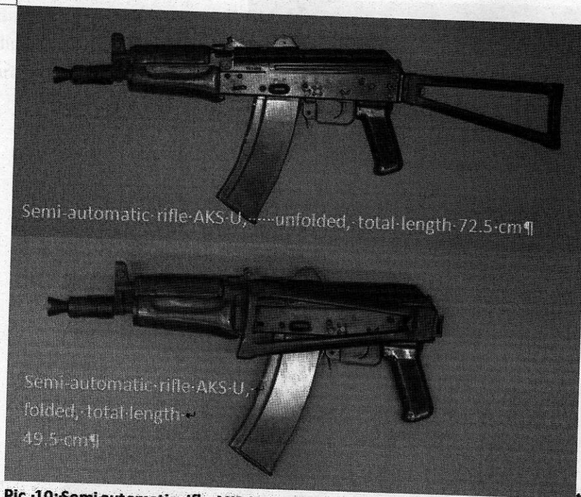
Pic.10: Semi-automatic rifle AKS-U, ca. 5.45mm x 39. The rifle can be reduced to a length below 60cm.
