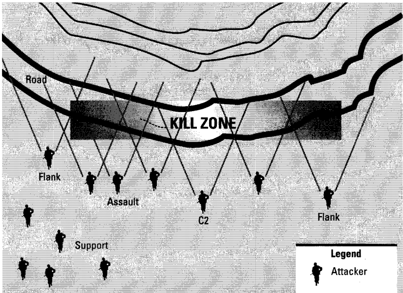
Figure II-3: Linear ambush.
