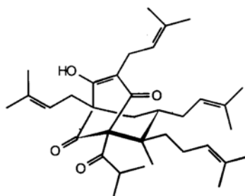
Hyperforin
