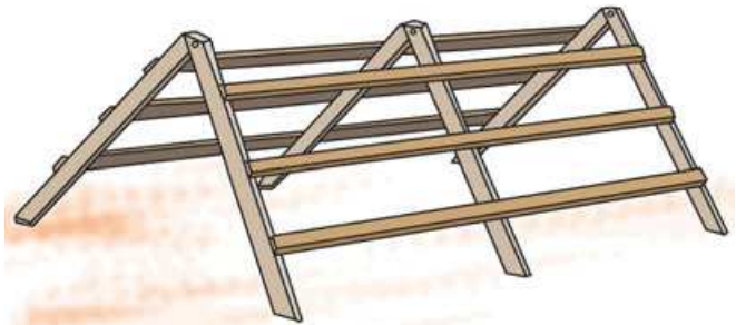
▲ A folding chicken roost.
