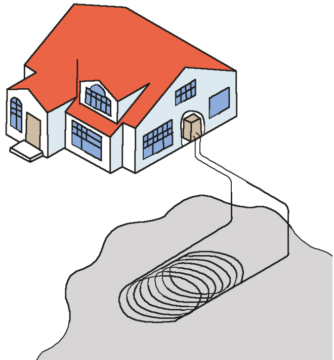
▲ A closed-loop pond/lake heat pump system.
