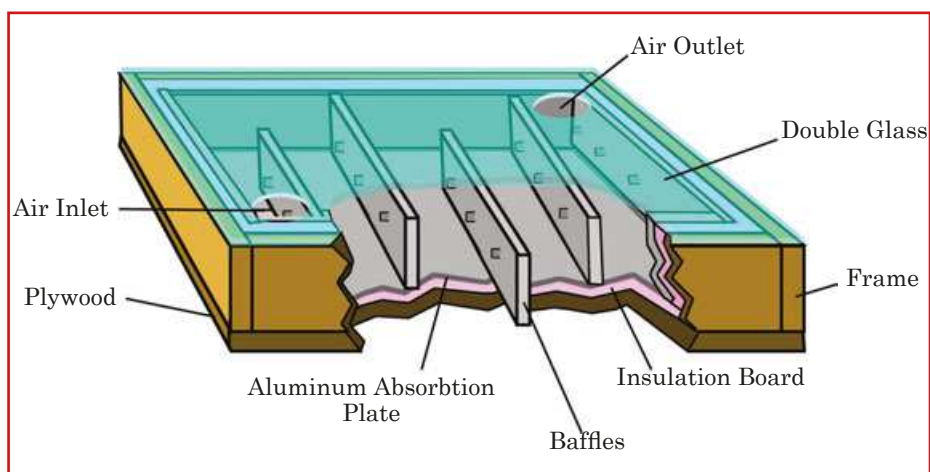
Alternate solar heating panel. ►
