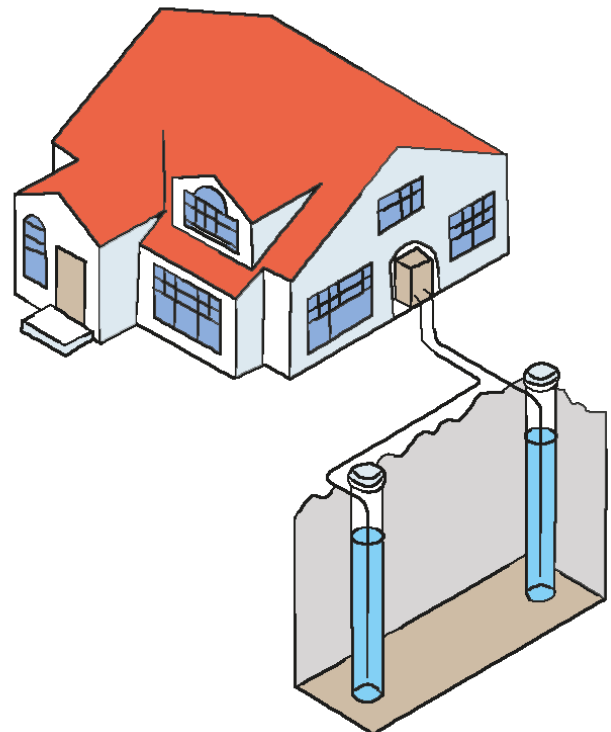
▲ An open-loop heat pump system.
