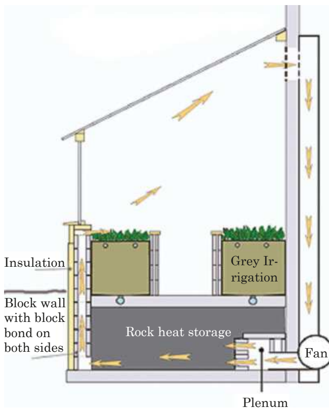
▼ An active cooling/passive heating greywater irrigated greenhouse.
