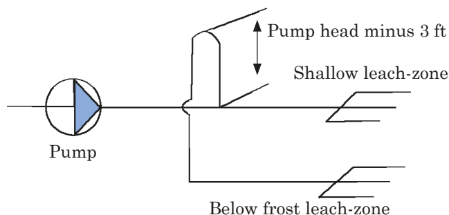
▲ About 3 feet of water is a good margin for this automatic switch system.
