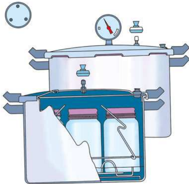
▲ A pressure canner.
