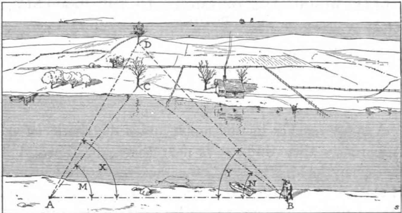
▲ Fig. 110. Determining distances to objects without measuring them.
