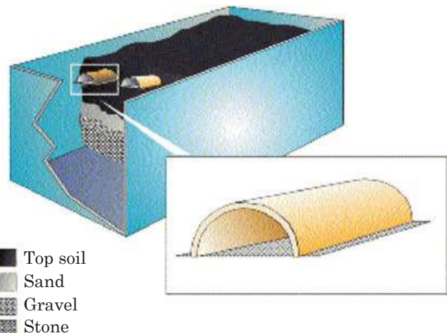
▲ A leaching chamber.
