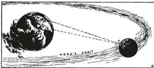
▲ Fig. 111. How the distance to the moon is measured. If the astronomer knows the length of the line AB and the size of the angles M and N, he can compute the distance to the point C.
