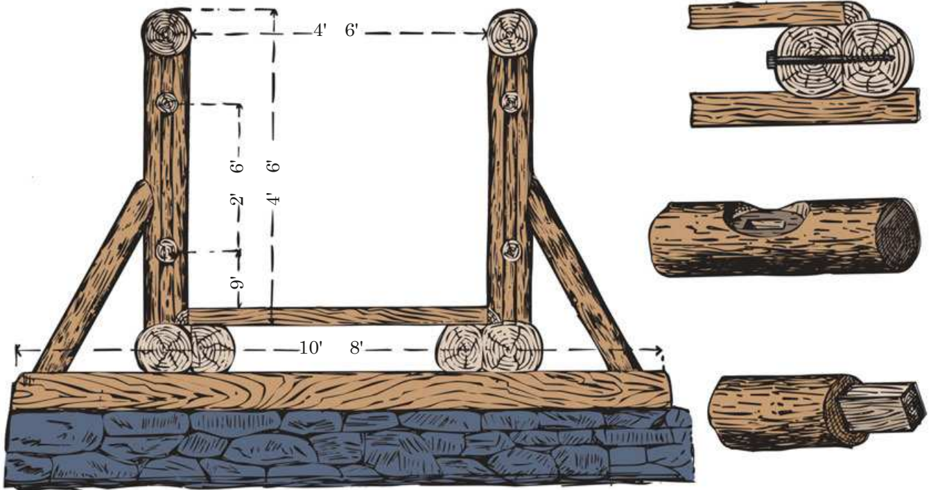
▲ A cross section of the footbridge.
