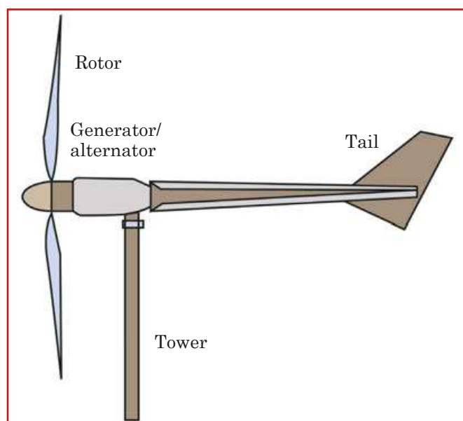
▲ The basic parts of a small wind electric system.
