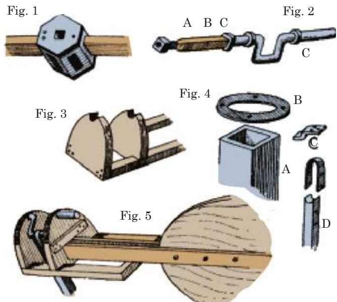
▲ Windmill pump details.
