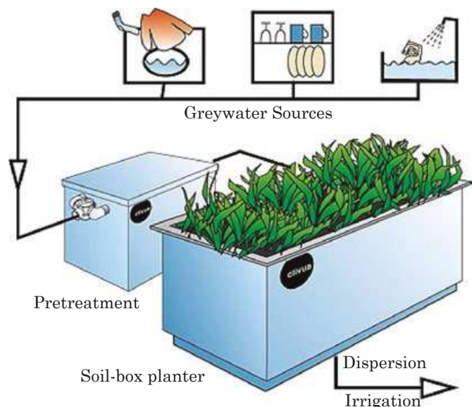
▲ Greywater irrigation.
