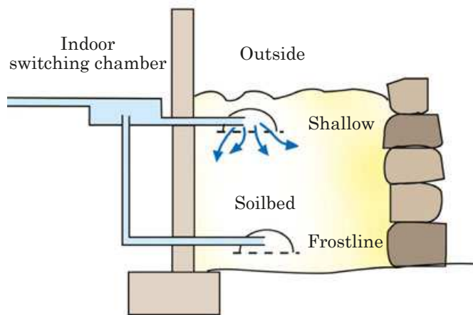
▲ An automatic switch system.
